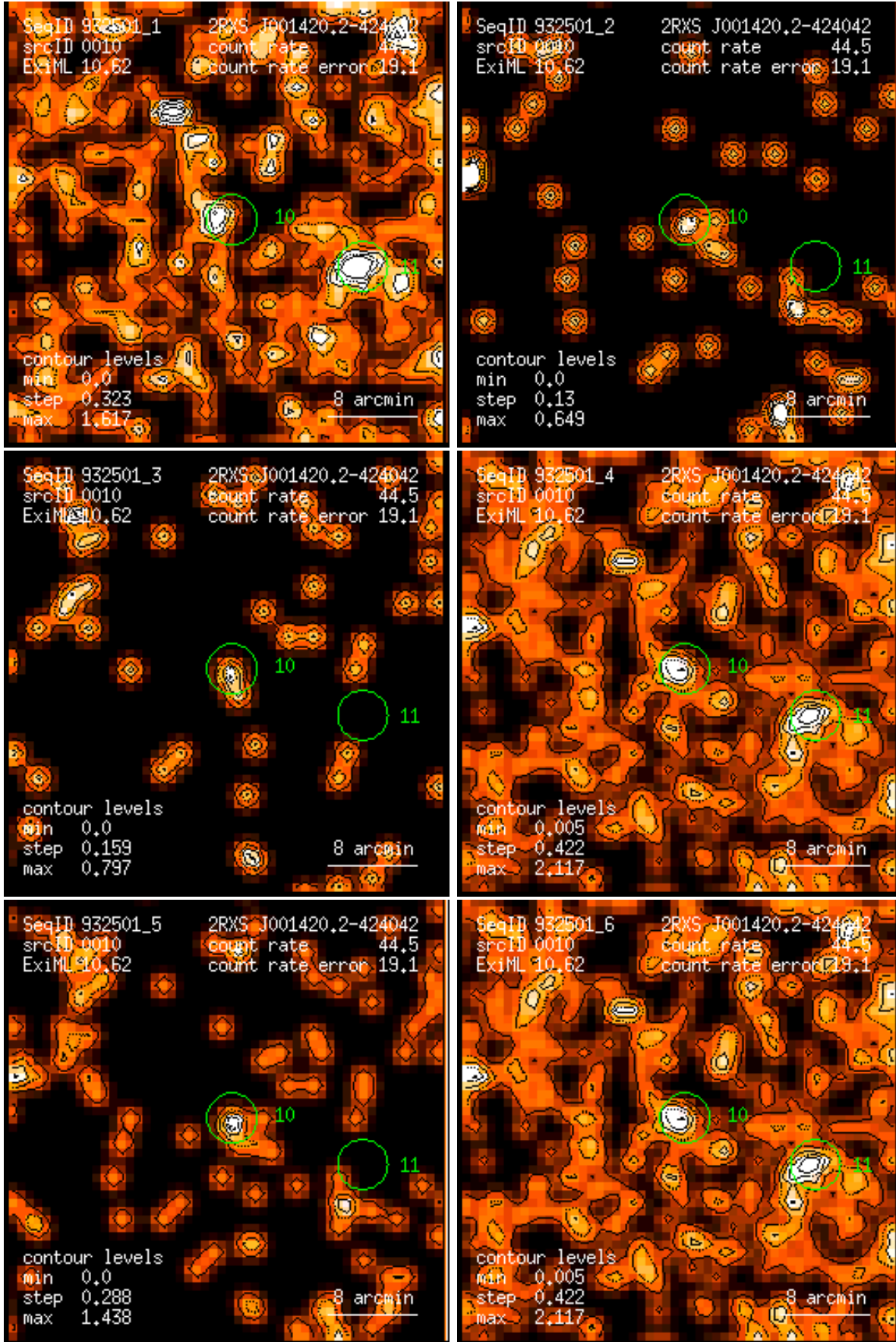
Figure 10: RASS 932501: detection 0010: band rate images, Gaussian filter: (1) PSPC channels 11 – 41, (2) 52 – 90, (3) 91 – 201, (4) 11 – 235, (5) 52 – 201, (6) 11 – 201. Broad band rates in counts/ks. Band rate contour levels in counts/ks/arcmin 2 .
