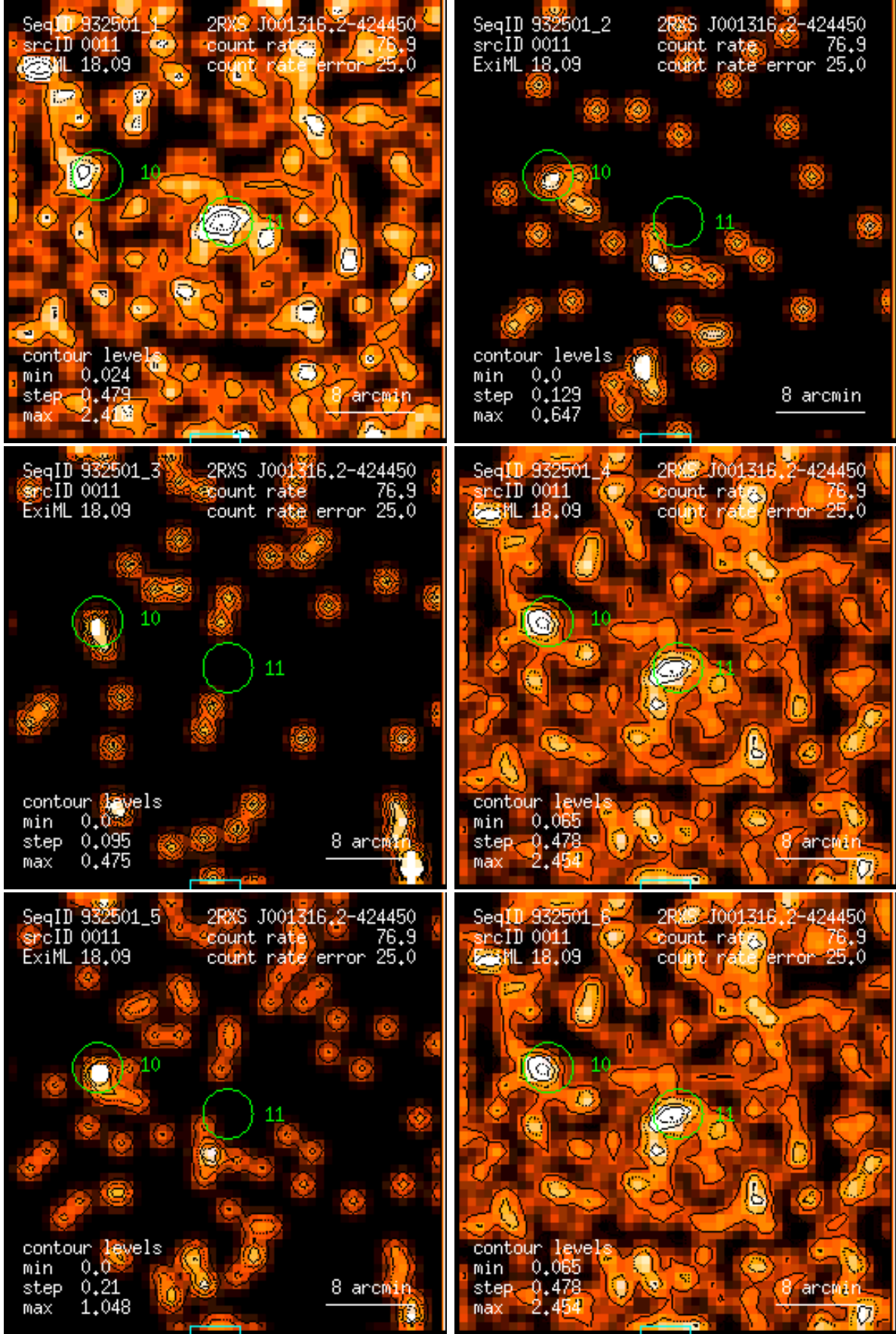
Figure 11: RASS 932501: detection 0011: band rate images, Gaussian filter: (1) PSPC channels 11 – 41, (2) 52 – 90, (3) 91 – 201, (4) 11 – 235, (5) 52 – 201, (6) 11 – 201. Broad band rates in counts/ks. Band rate contour levels in counts/ks/arcmin 2 .
