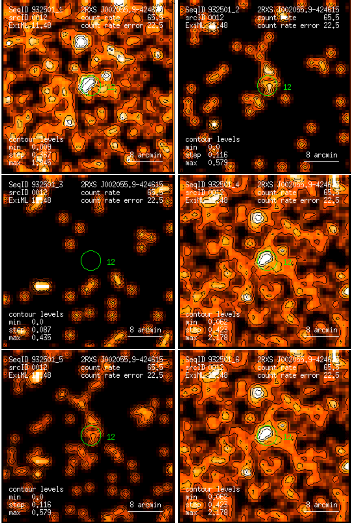
Figure 12: RASS 932501: detection 0012: band rate images, Gaussian filter: (1) PSPC channels 11 – 41, (2) 52 – 90, (3) 91 – 201, (4) 11 – 235, (5) 52 – 201, (6) 11 – 201. Broad band rates in counts/ks. Band rate contour levels in counts/ks/arcmin 2 .
