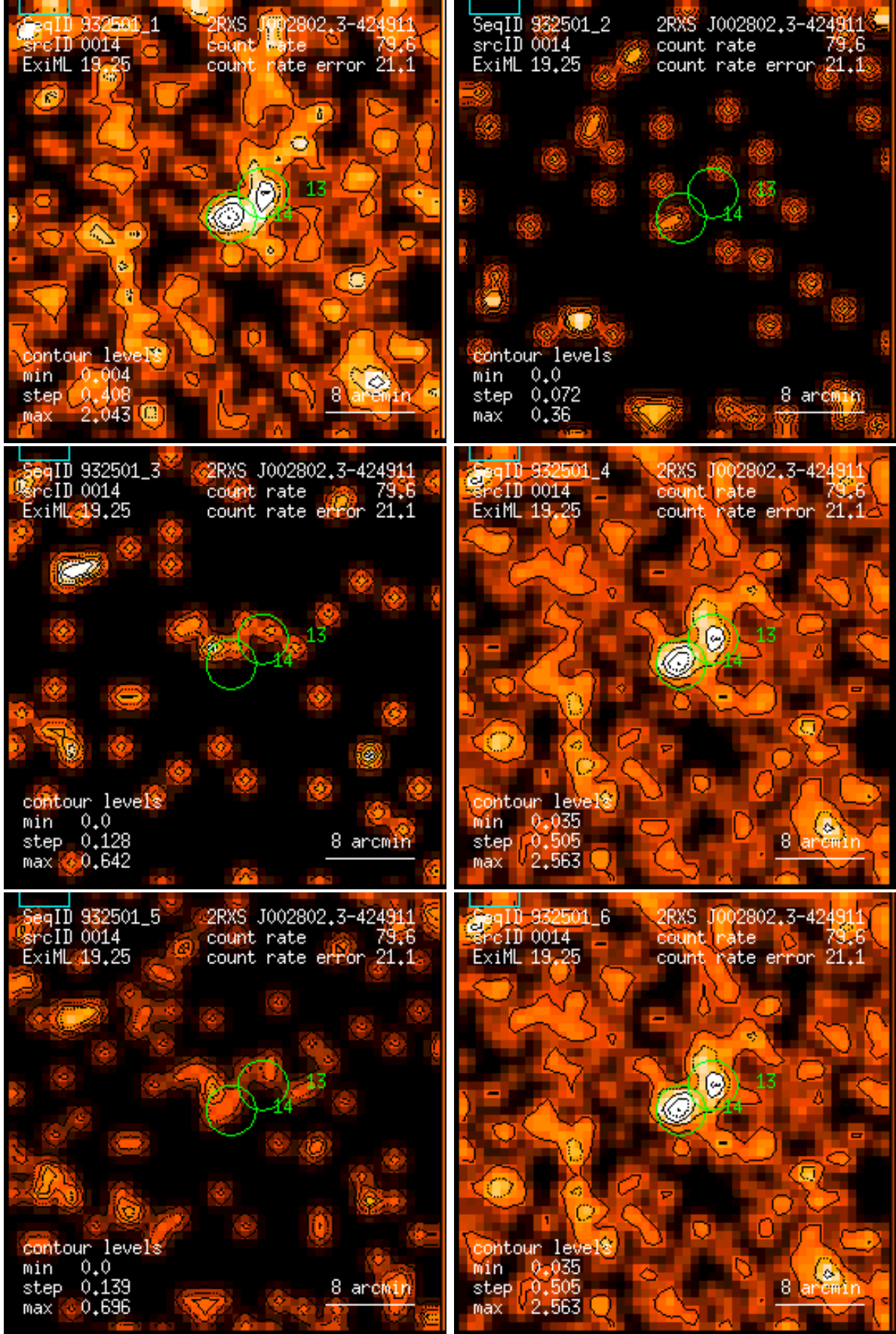
Figure 14: RASS 932501: detection 0014: band rate images, Gaussian filter: (1) PSPC channels 11 – 41, (2) 52 – 90, (3) 91 – 201, (4) 11 – 235, (5) 52 – 201, (6) 11 – 201. Broad band rates in counts/ks. Band rate contour levels in counts/ks/arcmin 2 .
