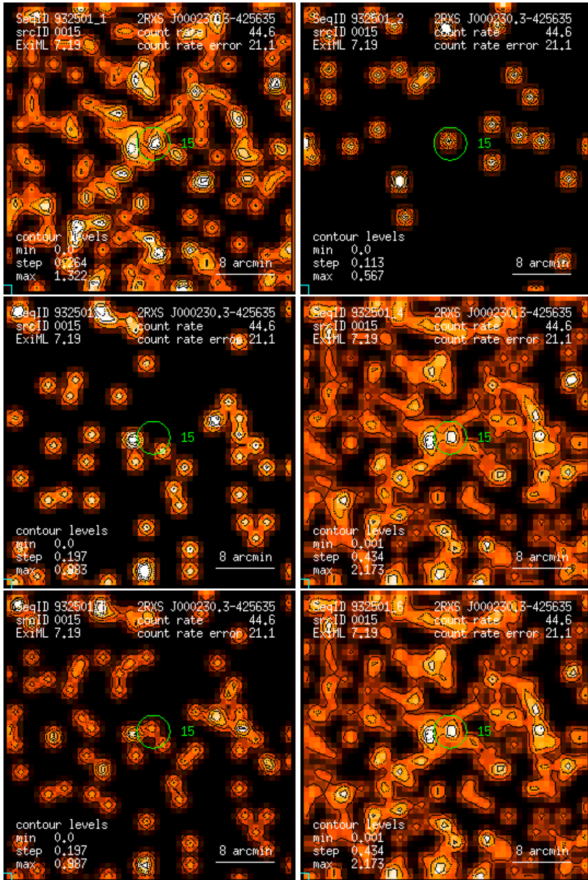
Figure 15: RASS 932501: detection 0015: band rate images, Gaussian filter: (1) PSPC channels 11 – 41, (2) 52 – 90, (3) 91 – 201, (4) 11 – 235, (5) 52 – 201, (6) 11 – 201. Broad band rates in counts/ks. Band rate contour levels in counts/ks/arcmin 2 .
