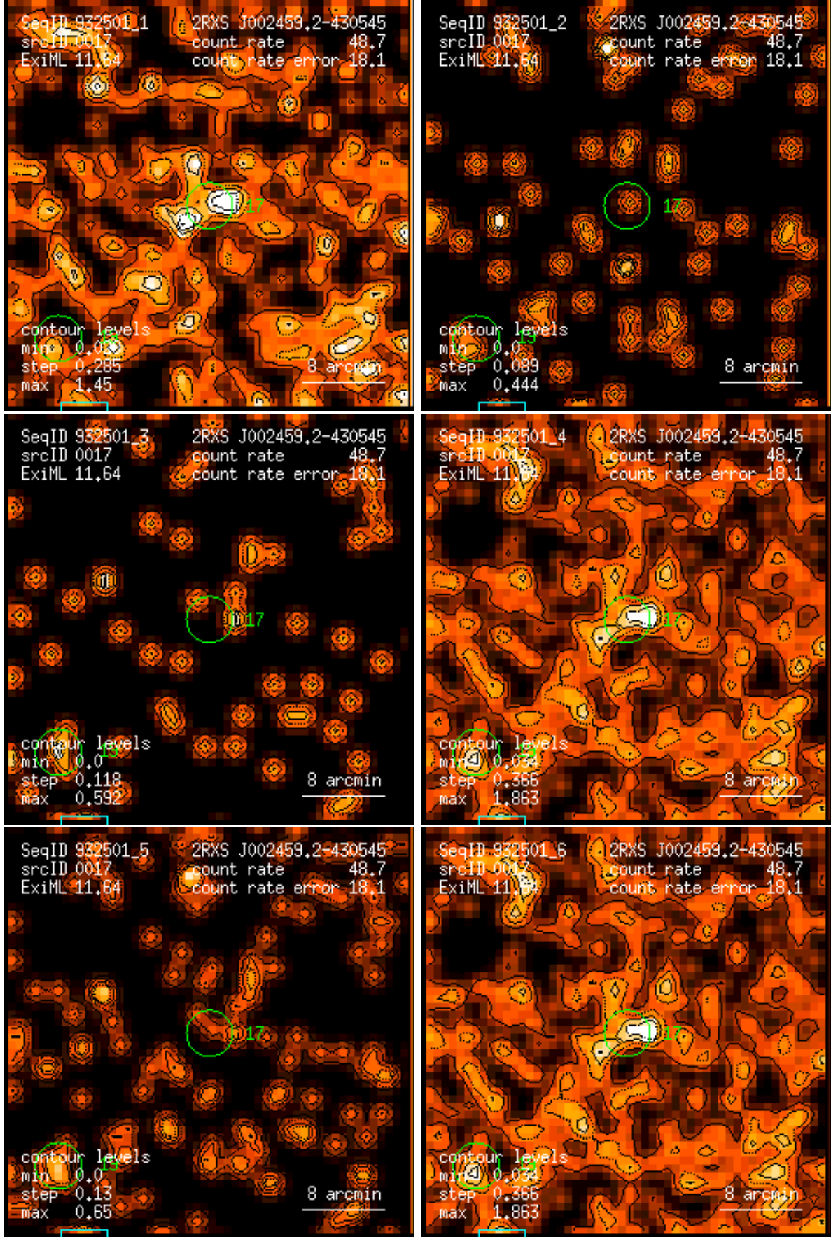
Figure 17: RASS 932501: detection 0017: band rate images, Gaussian filter: (1) PSPC channels 11 – 41, (2) 52 – 90, (3) 91 – 201, (4) 11 – 235, (5) 52 – 201, (6) 11 – 201. Broad band rates in counts/ks. Band rate contour levels in counts/ks/arcmin 2 .
