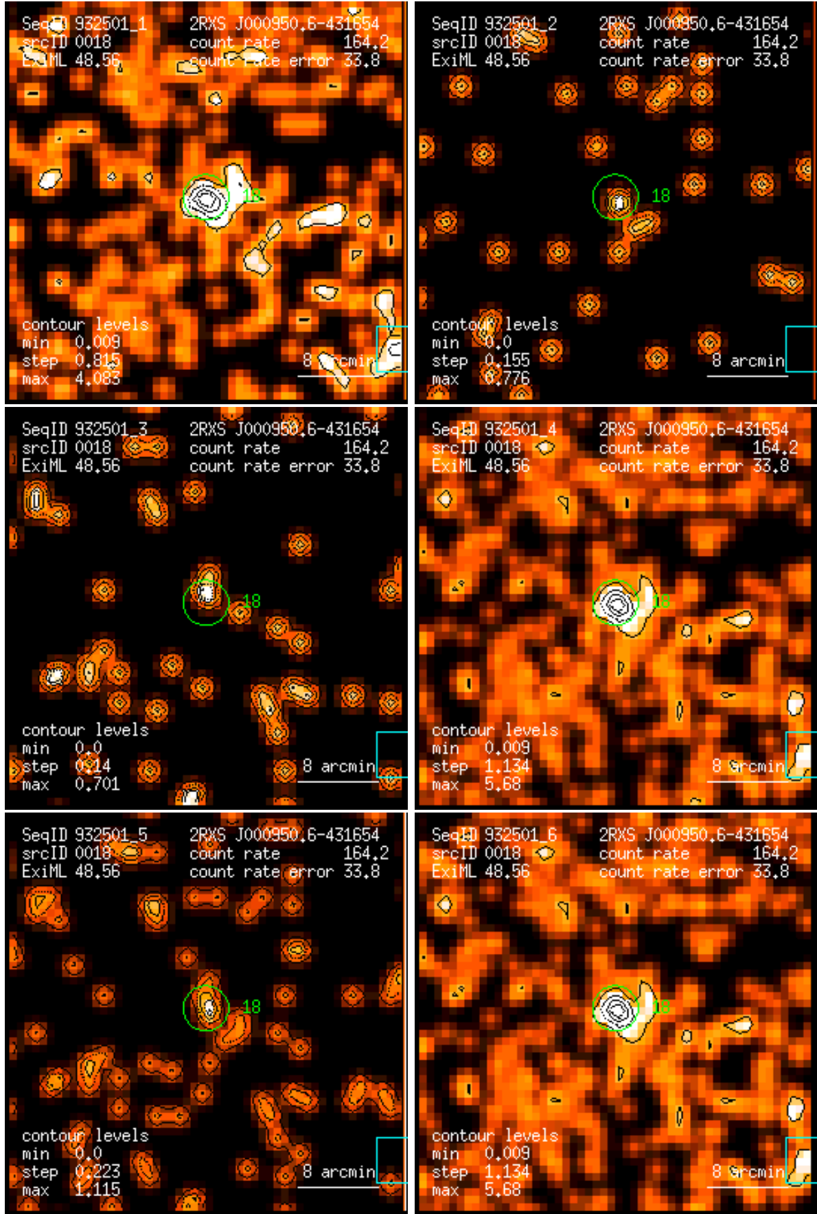
Figure 18: RASS 932501: detection 0018: band rate images, Gaussian filter: (1) PSPC channels 11 – 41, (2) 52 – 90, (3) 91 – 201, (4) 11 – 235, (5) 52 – 201, (6) 11 – 201. Broad band rates in counts/ks. Band rate contour levels in counts/ks/arcmin 2 .
