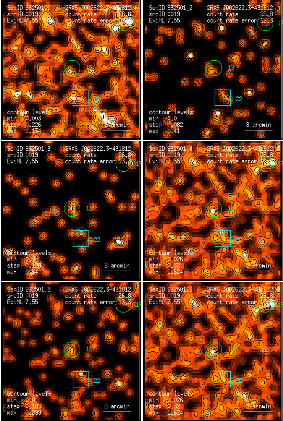
Figure 19: RASS 932501: detection 0019: band rate images, Gaussian filter: (1) PSPC channels 11 – 41, (2) 52 – 90, (3) 91 – 201, (4) 11 – 235, (5) 52 – 201, (6) 11 – 201. Broad band rates in counts/ks. Band rate contour levels in counts/ks/arcmin 2 .
