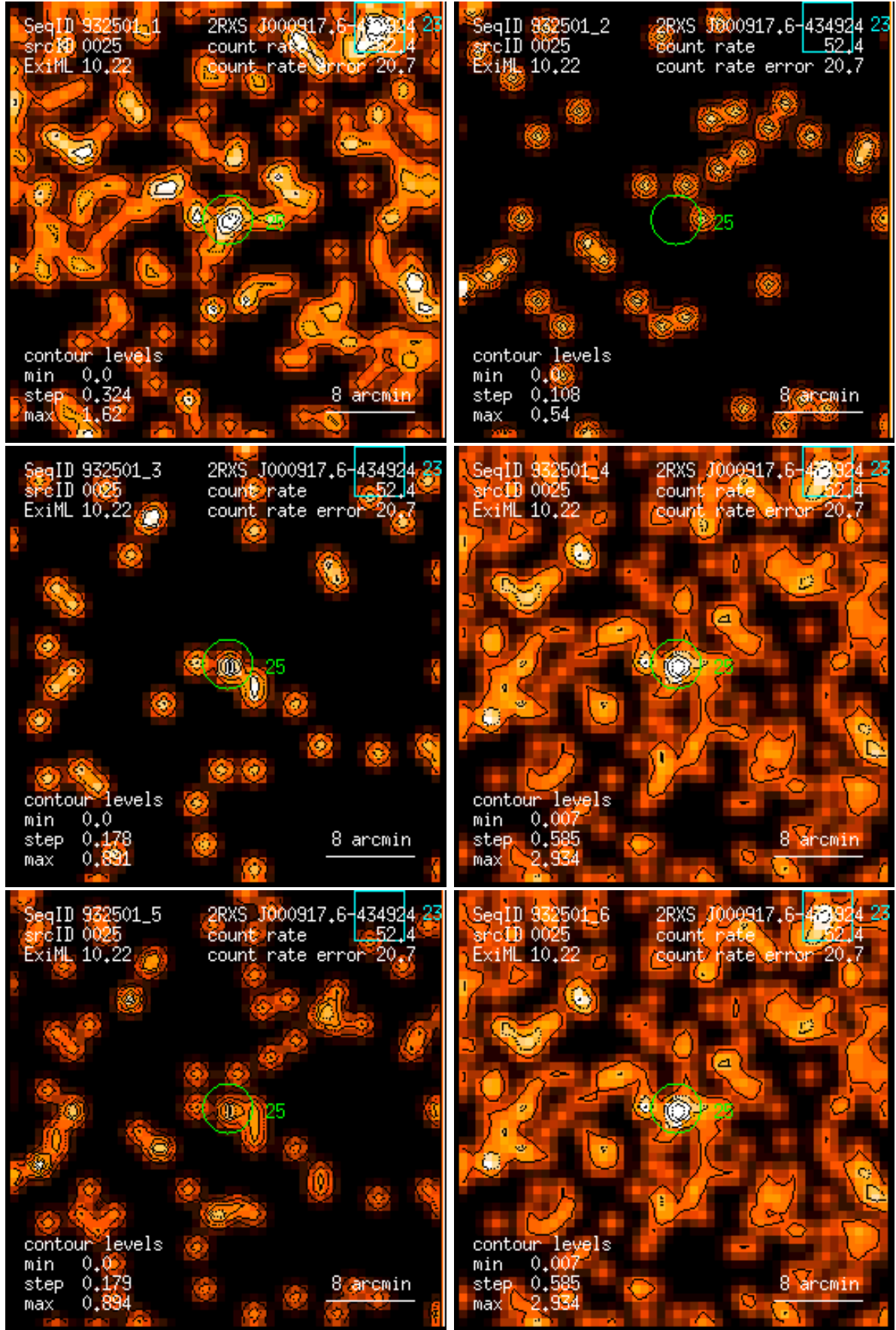
Figure 25: RASS 932501: detection 0025: band rate images, Gaussian filter: (1) PSPC channels 11 – 41, (2) 52 – 90, (3) 91 – 201, (4) 11 – 235, (5) 52 – 201, (6) 11 – 201. Broad band rates in counts/ks. Band rate contour levels in counts/ks/arcmin 2 .
