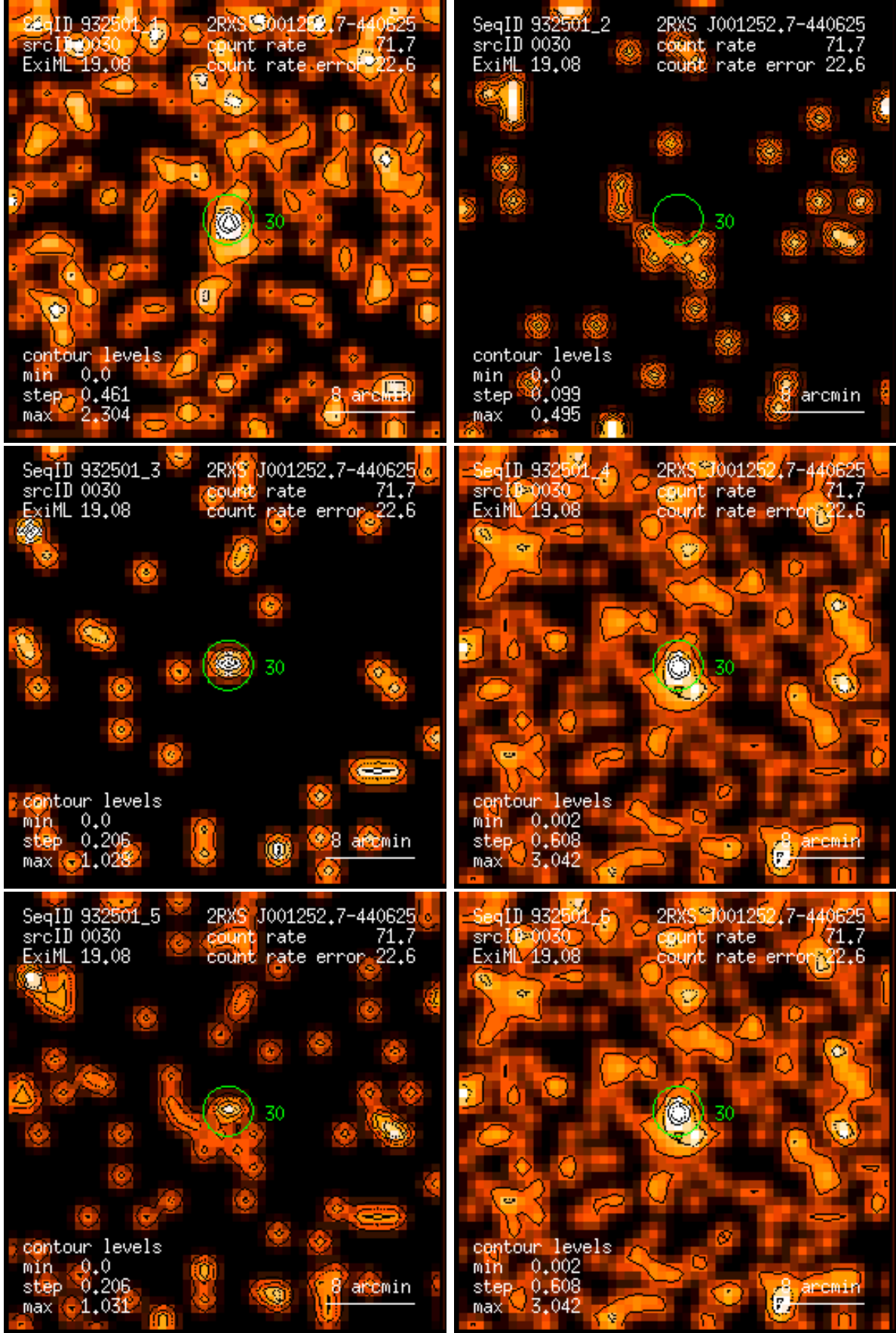
Figure 30: RASS 932501: detection 0030: band rate images, Gaussian filter: (1) PSPC channels 11 – 41, (2) 52 – 90, (3) 91 – 201, (4) 11 – 235, (5) 52 – 201, (6) 11 – 201. Broad band rates in counts/ks. Band rate contour levels in counts/ks/arcmin 2 .
