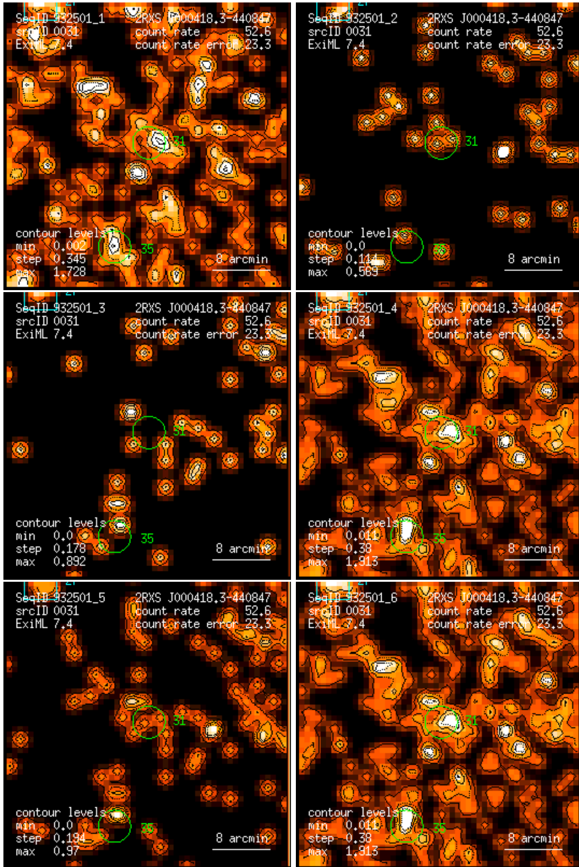
Figure 31: RASS 932501: detection 0031: band rate images, Gaussian filter: (1) PSPC channels 11 – 41, (2) 52 – 90, (3) 91 – 201, (4) 11 – 235, (5) 52 – 201, (6) 11 – 201. Broad band rates in counts/ks. Band rate contour levels in counts/ks/arcmin 2 .
