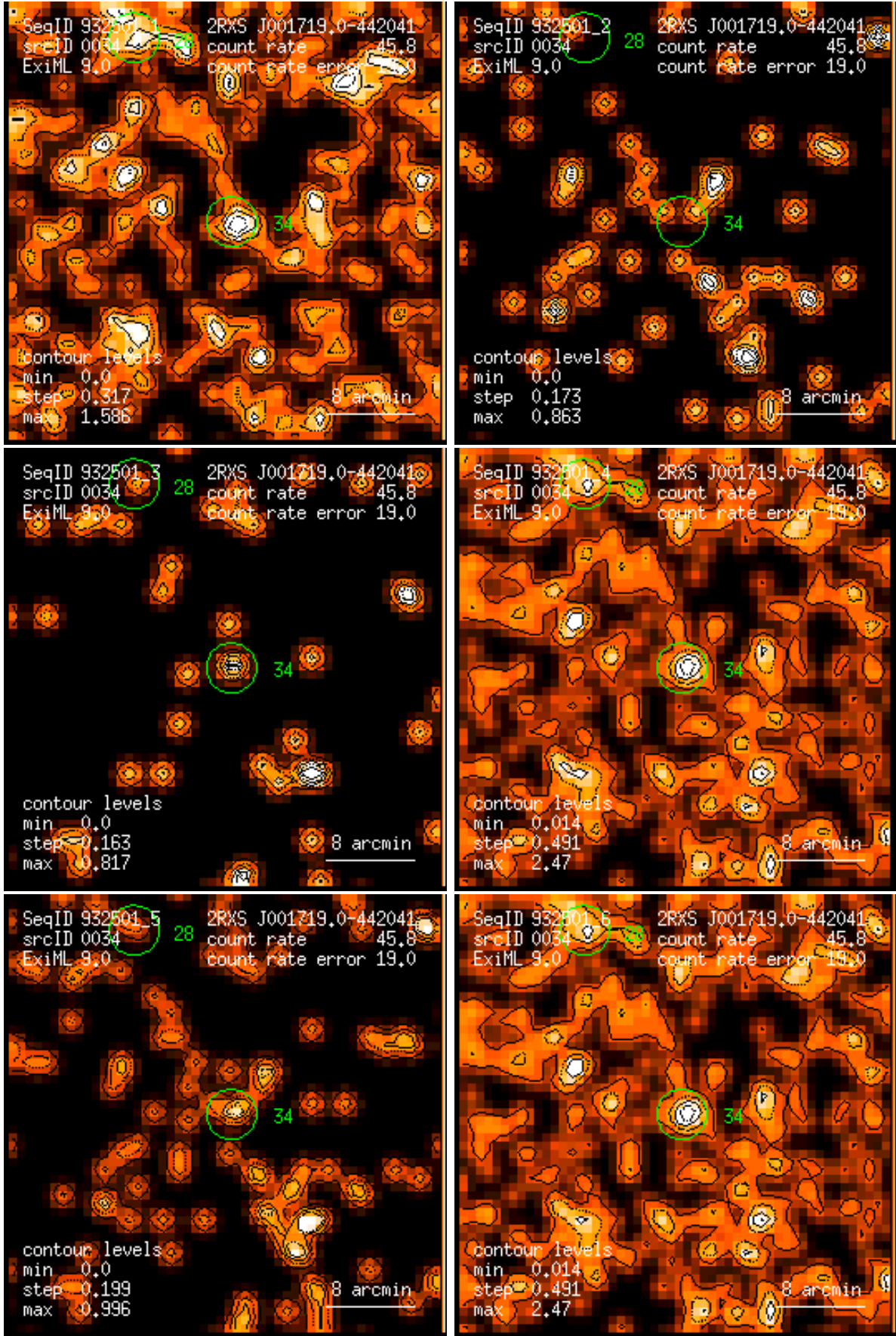
Figure 34: RASS 932501: detection 0034: band rate images, Gaussian filter: (1) PSPC channels 11 – 41, (2) 52 – 90, (3) 91 – 201, (4) 11 – 235, (5) 52 – 201, (6) 11 – 201. Broad band rates in counts/ks. Band rate contour levels in counts/ks/arcmin 2 .
