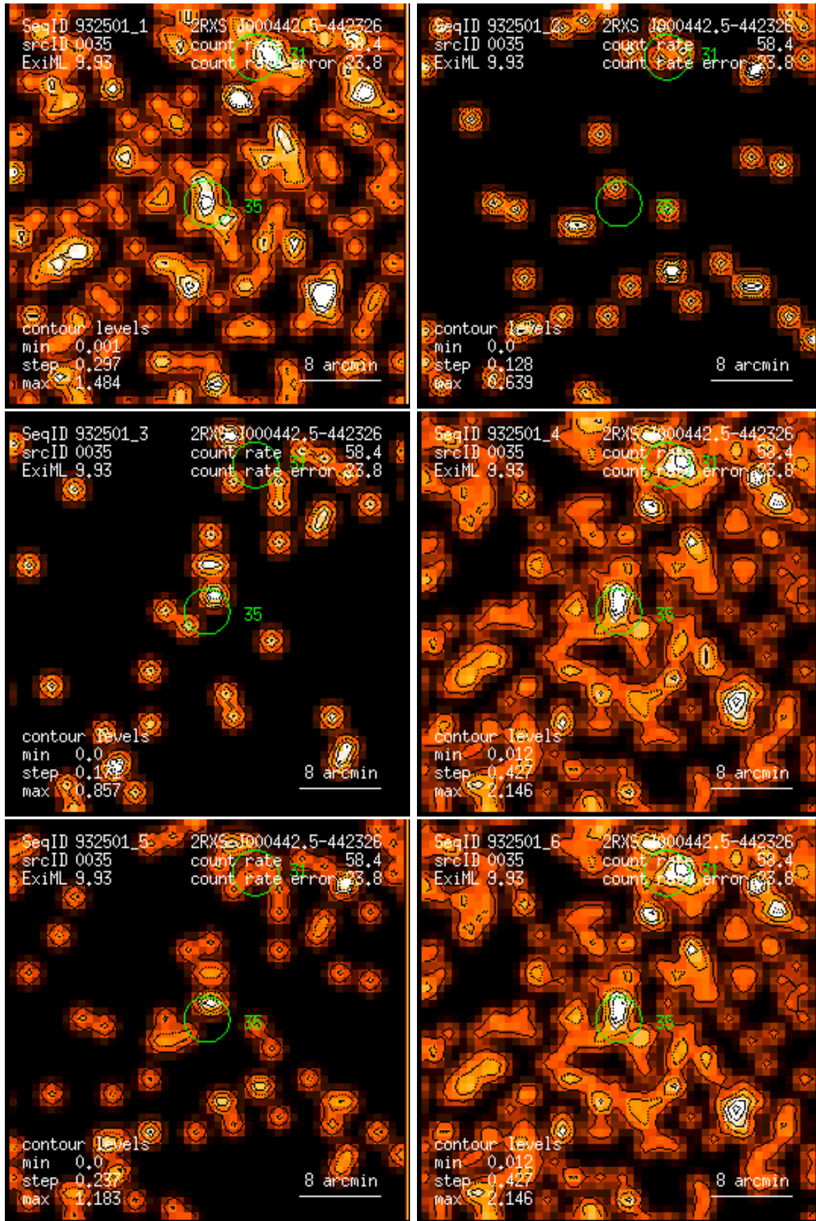
Figure 35: RASS 932501: detection 0035: band rate images, Gaussian filter: (1) PSPC channels 11 – 41, (2) 52 – 90, (3) 91 – 201, (4) 11 – 235, (5) 52 – 201, (6) 11 – 201. Broad band rates in counts/ks. Band rate contour levels in counts/ks/arcmin 2 .
