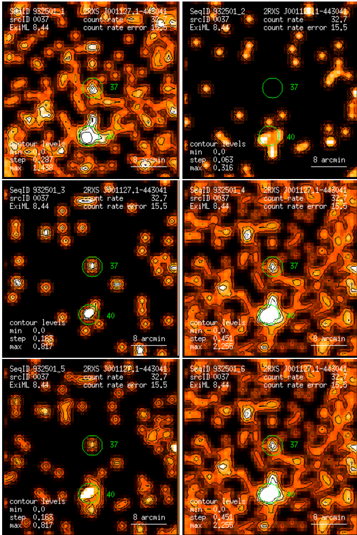
Figure 37: RASS 932501: detection 0037: band rate images, Gaussian filter: (1) PSPC channels 11 – 41, (2) 52 – 90, (3) 91 – 201, (4) 11 – 235, (5) 52 – 201, (6) 11 – 201. Broad band rates in counts/ks. Band rate contour levels in counts/ks/arcmin 2 .
