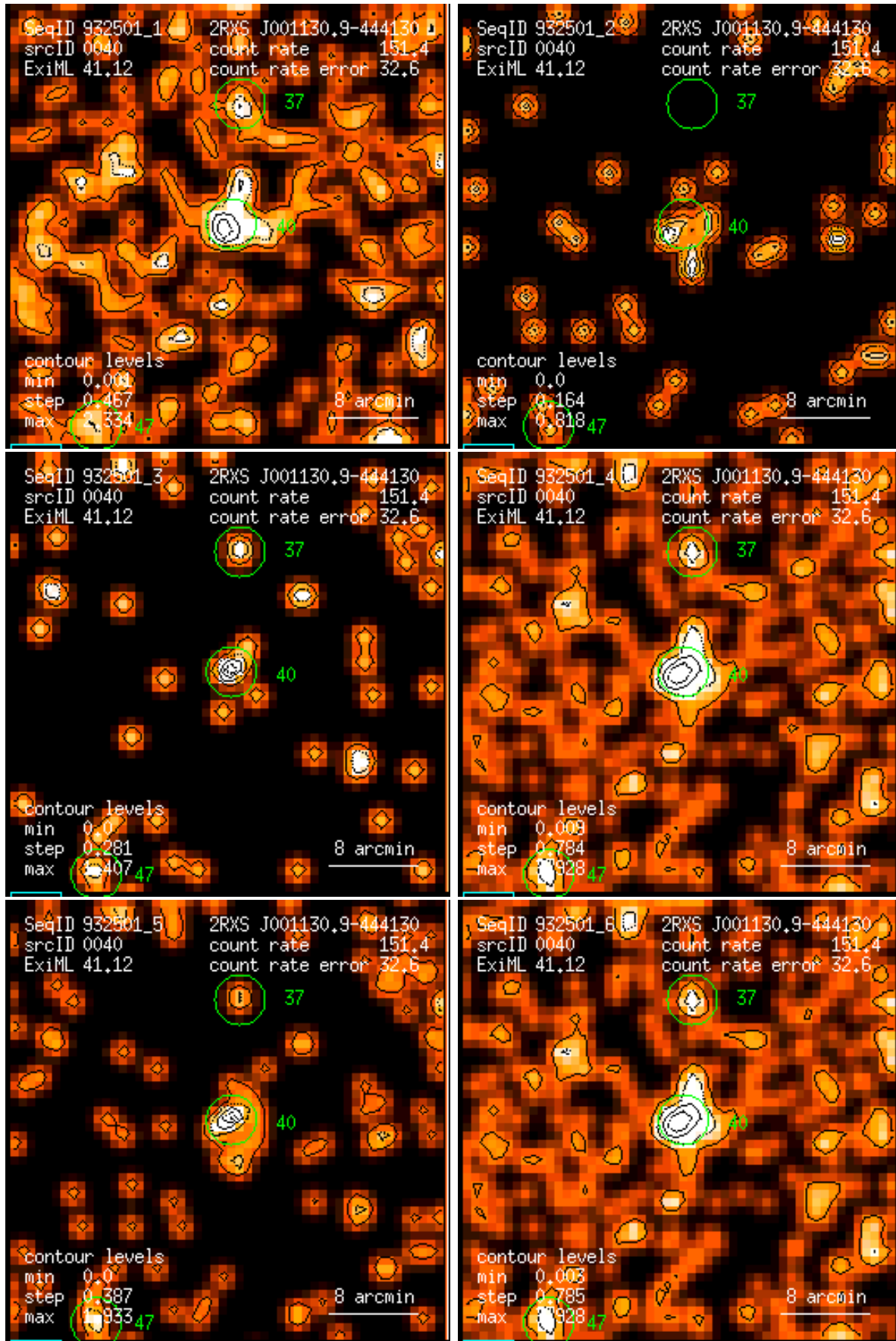
Figure 40: RASS 932501: detection 0040: band rate images, Gaussian filter: (1) PSPC channels 11 – 41, (2) 52 – 90, (3) 91 – 201, (4) 11 – 235, (5) 52 – 201, (6) 11 – 201. Broad band rates in counts/ks. Band rate contour levels in counts/ks/arcmin 2 .
