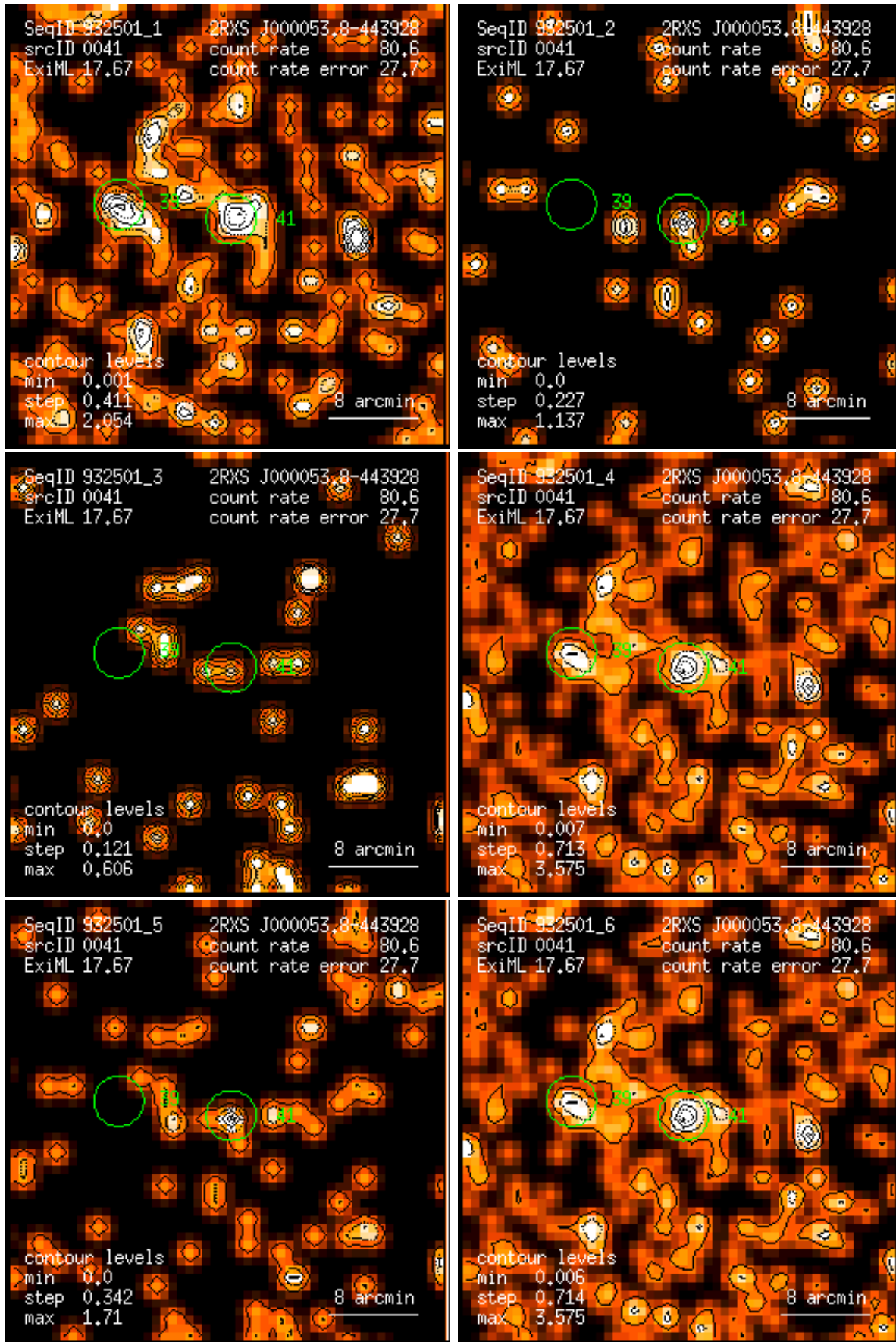
Figure 41: RASS 932501: detection 0041: band rate images, Gaussian filter: (1) PSPC channels 11 – 41, (2) 52 – 90, (3) 91 – 201, (4) 11 – 235, (5) 52 – 201, (6) 11 – 201. Broad band rates in counts/ks. Band rate contour levels in counts/ks/arcmin 2 .
