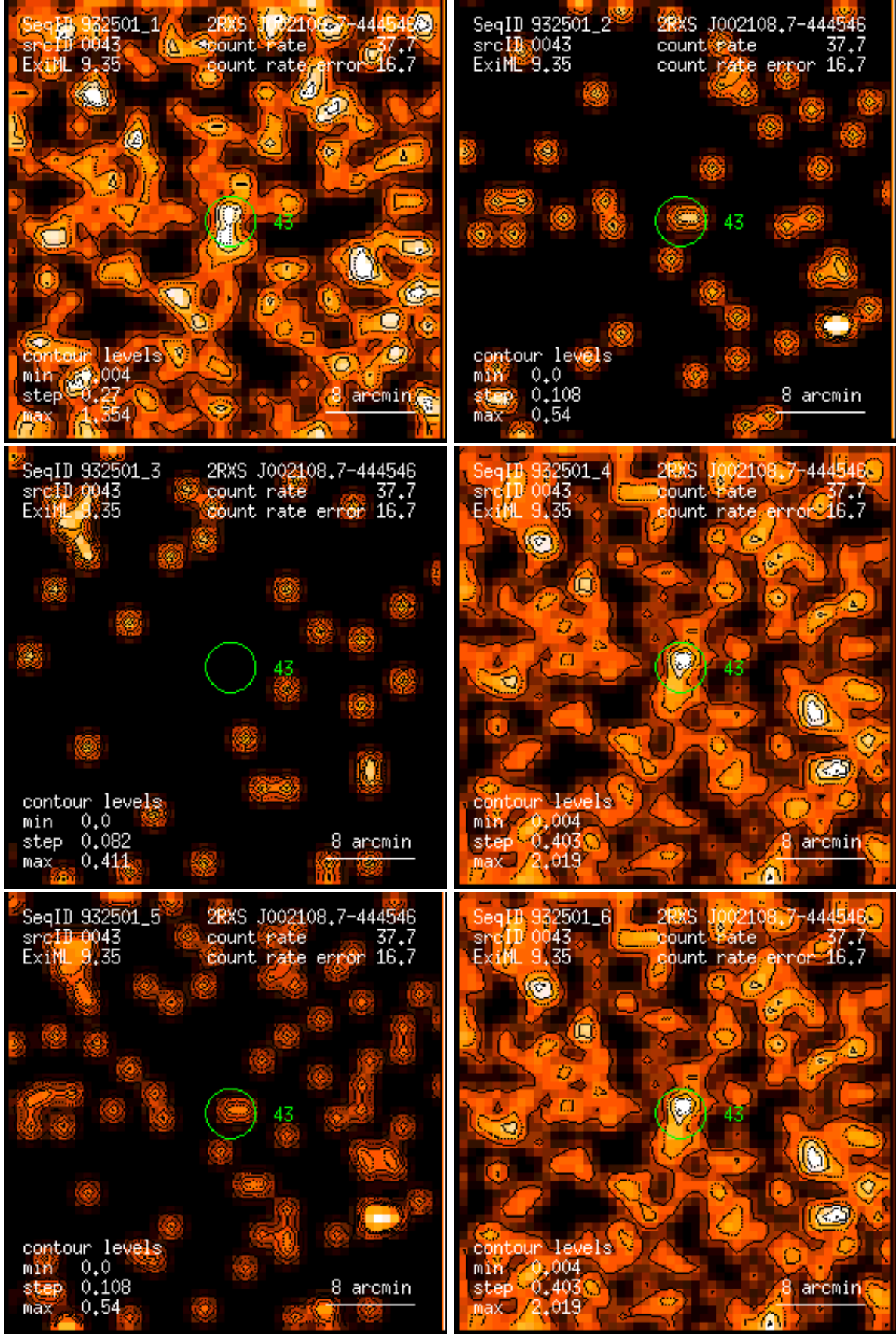
Figure 43: RASS 932501: detection 0043: band rate images, Gaussian filter: (1) PSPC channels 11 – 41, (2) 52 – 90, (3) 91 – 201, (4) 11 – 235, (5) 52 – 201, (6) 11 – 201. Broad band rates in counts/ks. Band rate contour levels in counts/ks/arcmin 2 .
