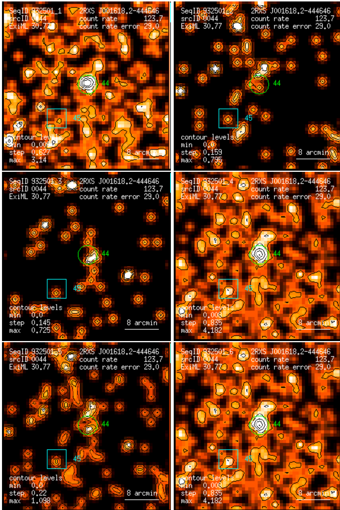
Figure 44: RASS 932501: detection 0044: band rate images, Gaussian filter: (1) PSPC channels 11 – 41, (2) 52 – 90, (3) 91 – 201, (4) 11 – 235, (5) 52 – 201, (6) 11 – 201. Broad band rates in counts/ks. Band rate contour levels in counts/ks/arcmin 2 .
