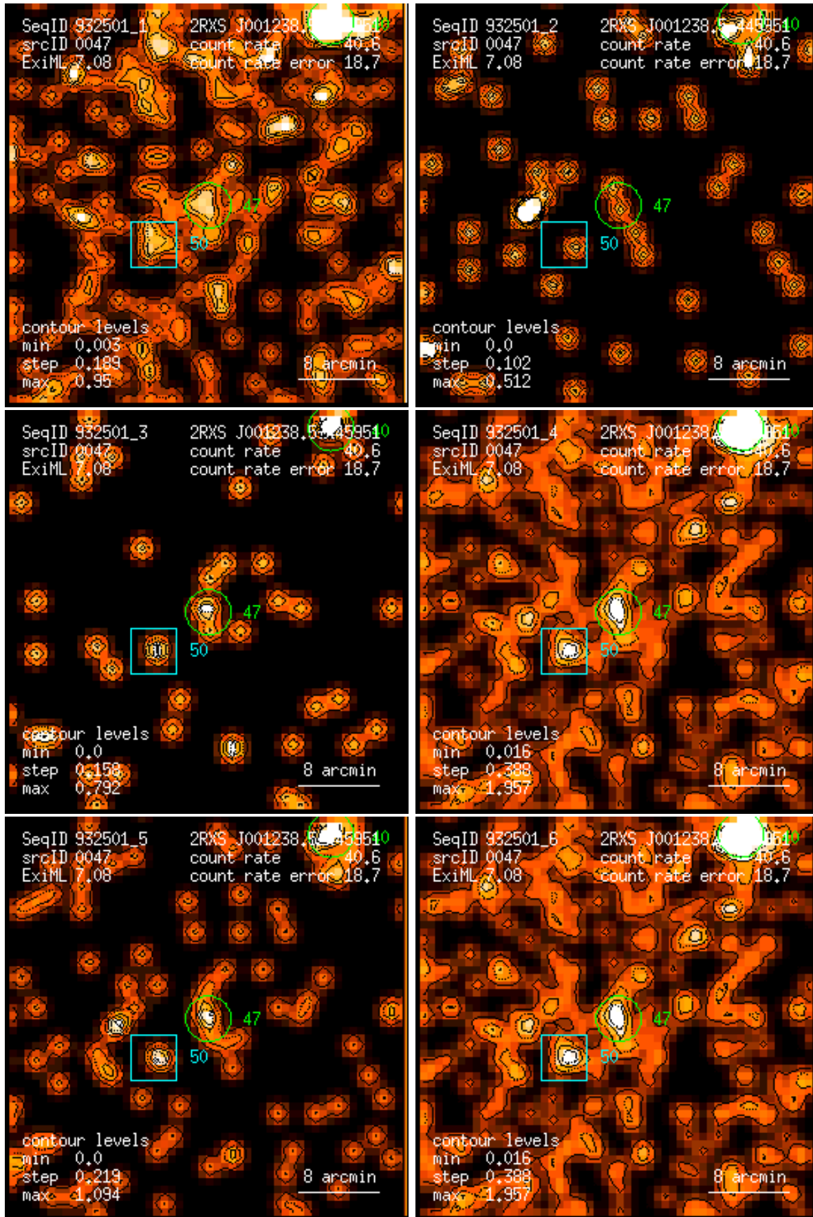
Figure 47: RASS 932501: detection 0047: band rate images, Gaussian filter: (1) PSPC channels 11 – 41, (2) 52 – 90, (3) 91 – 201, (4) 11 – 235, (5) 52 – 201, (6) 11 – 201. Broad band rates in counts/ks. Band rate contour levels in counts/ks/arcmin 2 .
