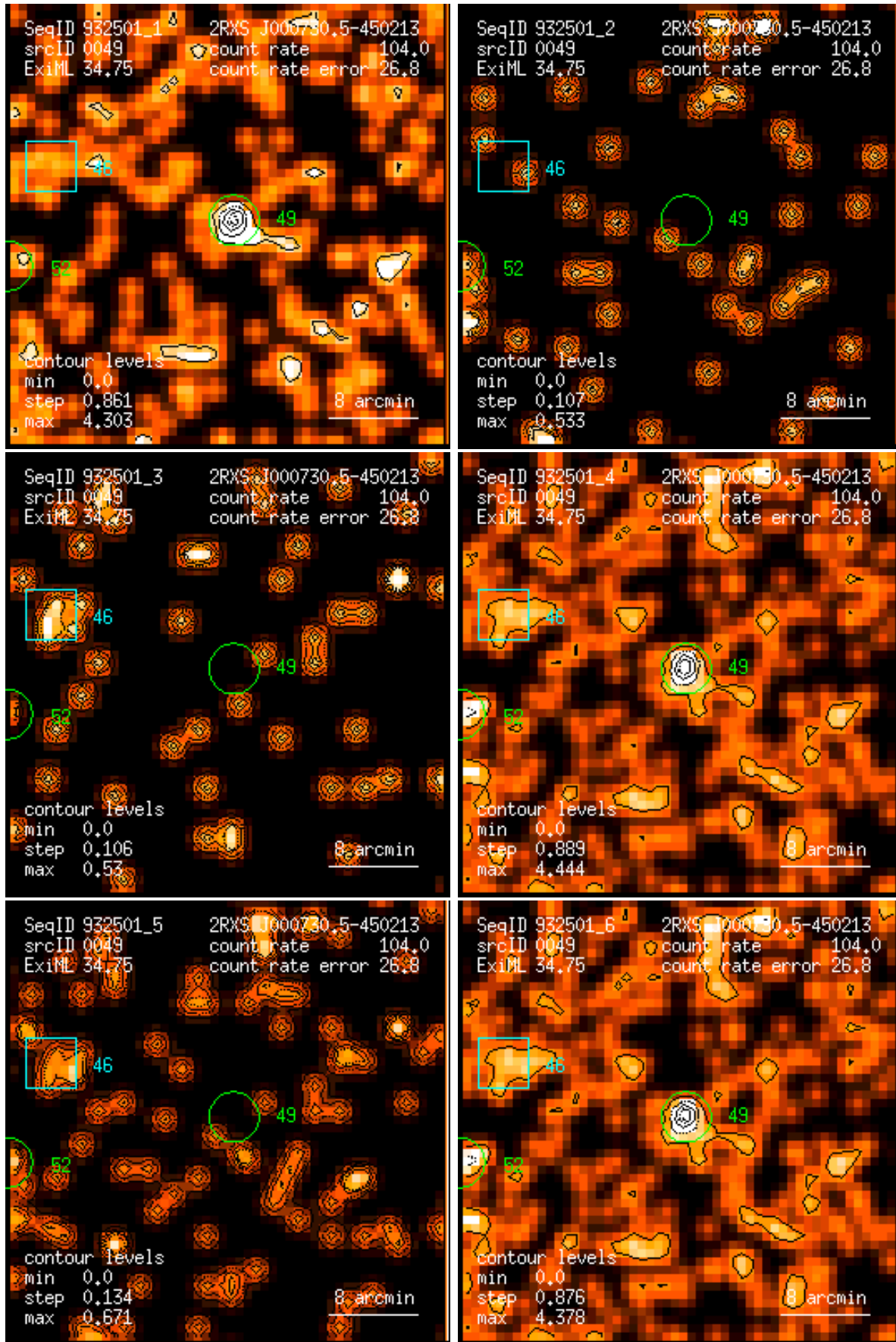
Figure 49: RASS 932501: detection 0049: band rate images, Gaussian filter: (1) PSPC channels 11 – 41, (2) 52 – 90, (3) 91 – 201, (4) 11 – 235, (5) 52 – 201, (6) 11 – 201. Broad band rates in counts/ks. Band rate contour levels in counts/ks/arcmin 2 .
