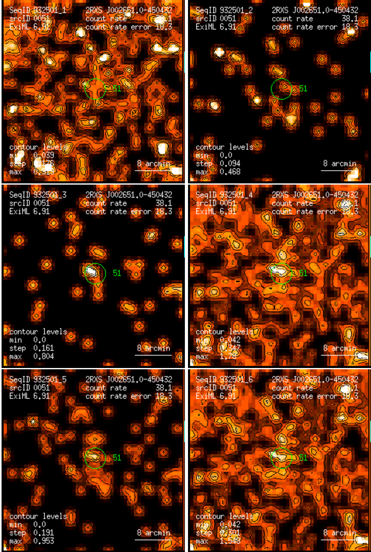
Figure 51: RASS 932501: detection 0051: band rate images, Gaussian filter: (1) PSPC channels 11 – 41, (2) 52 – 90, (3) 91 – 201, (4) 11 – 235, (5) 52 – 201, (6) 11 – 201. Broad band rates in counts/ks. Band rate contour levels in counts/ks/arcmin 2 .
