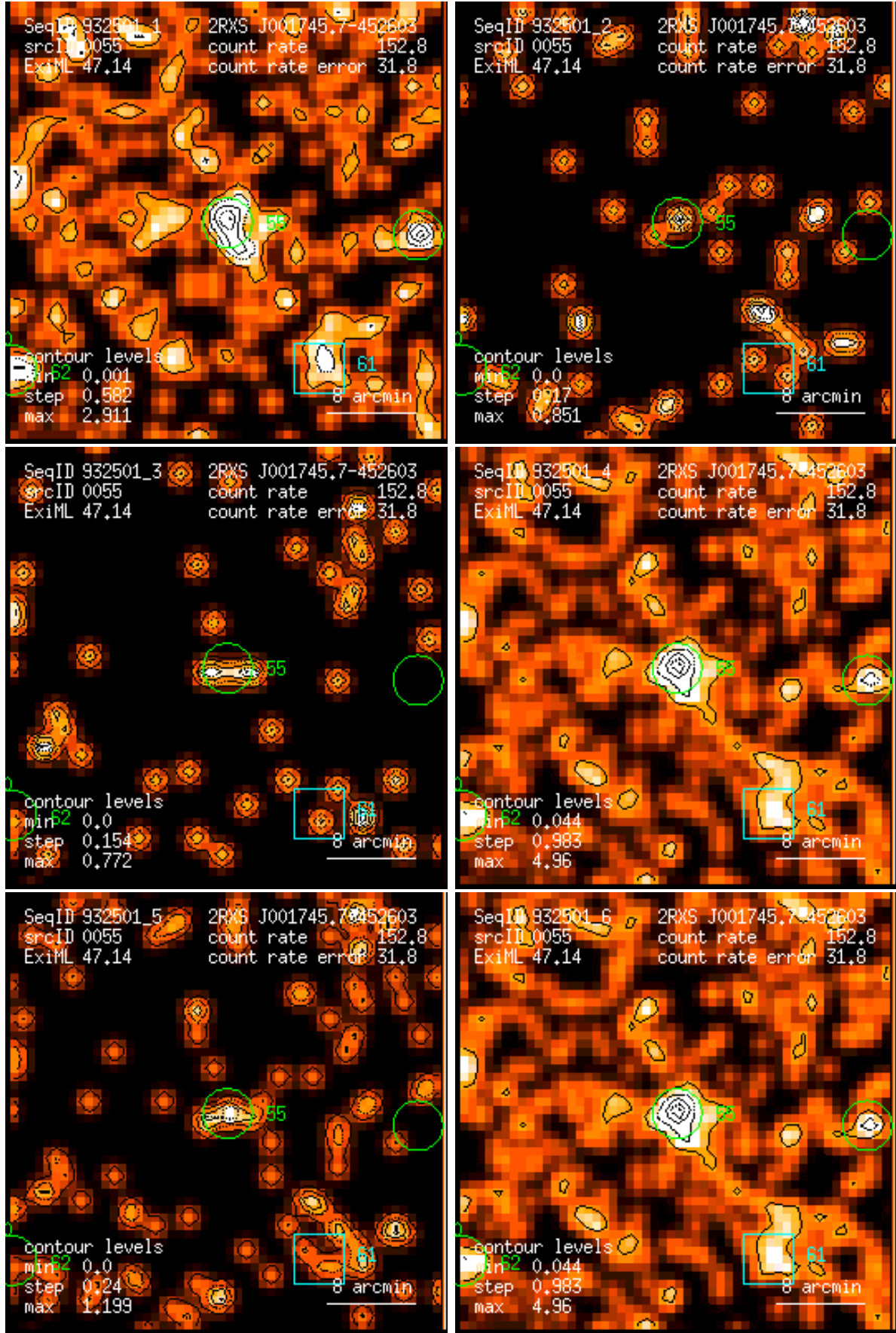
Figure 55: RASS 932501: detection 0055: band rate images, Gaussian filter: (1) PSPC channels 11 – 41, (2) 52 – 90, (3) 91 – 201, (4) 11 – 235, (5) 52 – 201, (6) 11 – 201. Broad band rates in counts/ks. Band rate contour levels in counts/ks/arcmin 2 .
