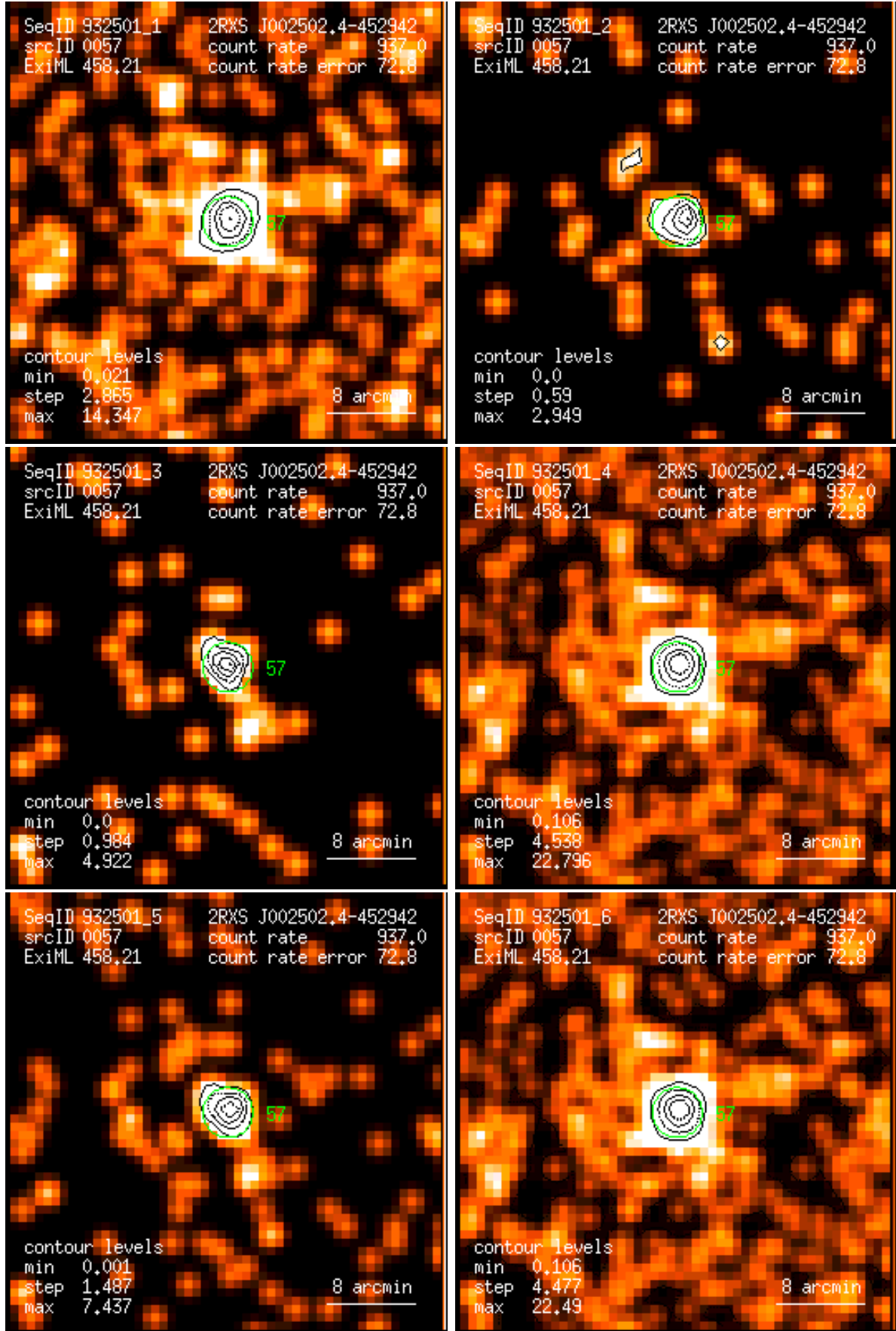
Figure 57: RASS 932501: detection 0057: band rate images, Gaussian filter: (1) PSPC channels 11 – 41, (2) 52 – 90, (3) 91 – 201, (4) 11 – 235, (5) 52 – 201, (6) 11 – 201. Broad band rates in counts/ks. Band rate contour levels in counts/ks/arcmin 2 .
