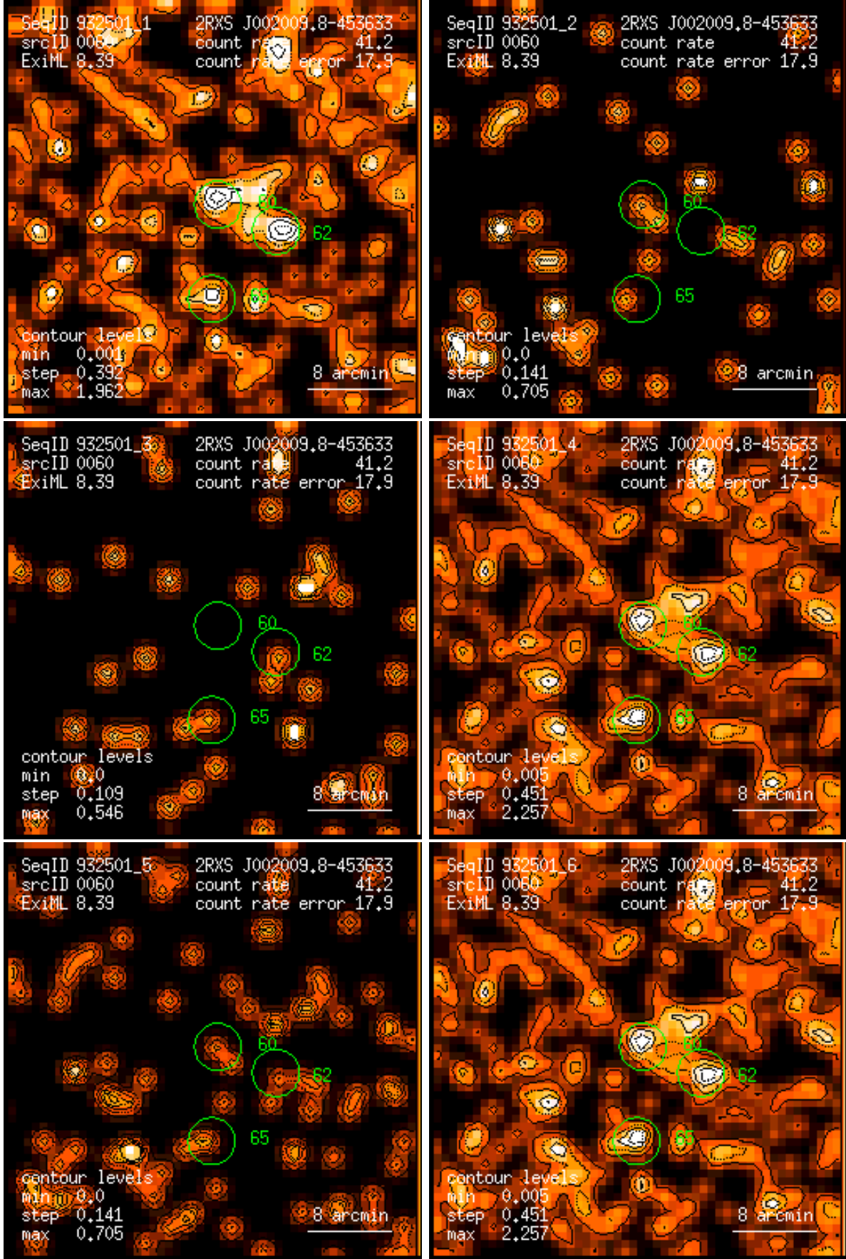
Figure 60: RASS 932501: detection 0060: band rate images, Gaussian filter: (1) PSPC channels 11 – 41, (2) 52 – 90, (3) 91 – 201, (4) 11 – 235, (5) 52 – 201, (6) 11 – 201. Broad band rates in counts/ks. Band rate contour levels in counts/ks/arcmin 2 .
