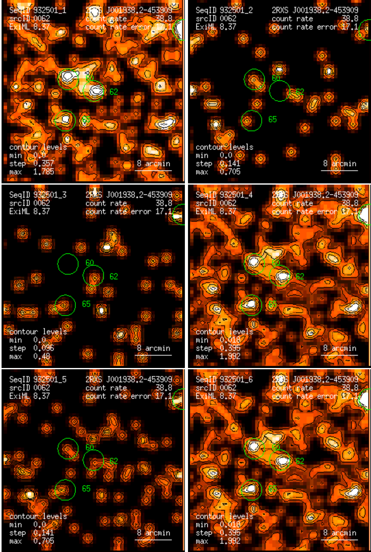
Figure 62: RASS 932501: detection 0062: band rate images, Gaussian filter: (1) PSPC channels 11 – 41, (2) 52 – 90, (3) 91 – 201, (4) 11 – 235, (5) 52 – 201, (6) 11 – 201. Broad band rates in counts/ks. Band rate contour levels in counts/ks/arcmin 2 .
