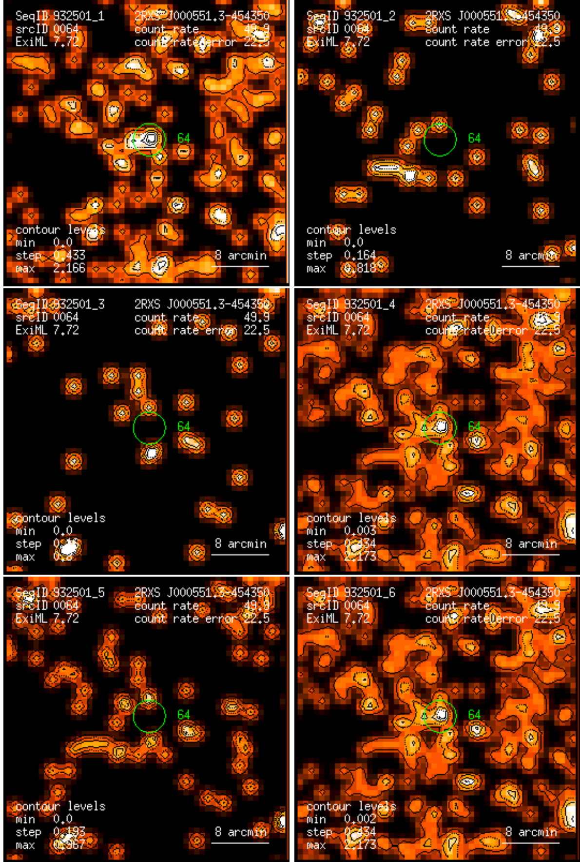
Figure 64: RASS 932501: detection 0064: band rate images, Gaussian filter: (1) PSPC channels 11 – 41, (2) 52 – 90, (3) 91 – 201, (4) 11 – 235, (5) 52 – 201, (6) 11 – 201. Broad band rates in counts/ks. Band rate contour levels in counts/ks/arcmin 2 .
