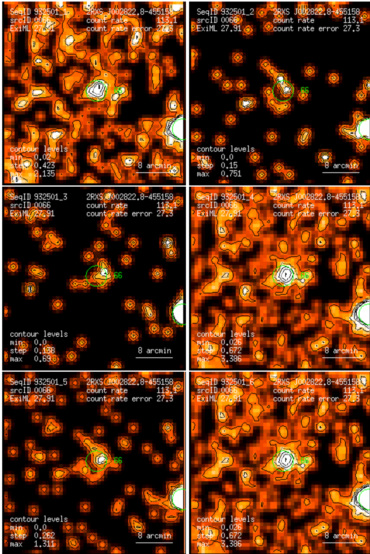
Figure 66: RASS 932501: detection 0066: band rate images, Gaussian filter: (1) PSPC channels 11 – 41, (2) 52 – 90, (3) 91 – 201, (4) 11 – 235, (5) 52 – 201, (6) 11 – 201. Broad band rates in counts/ks. Band rate contour levels in counts/ks/arcmin 2 .
