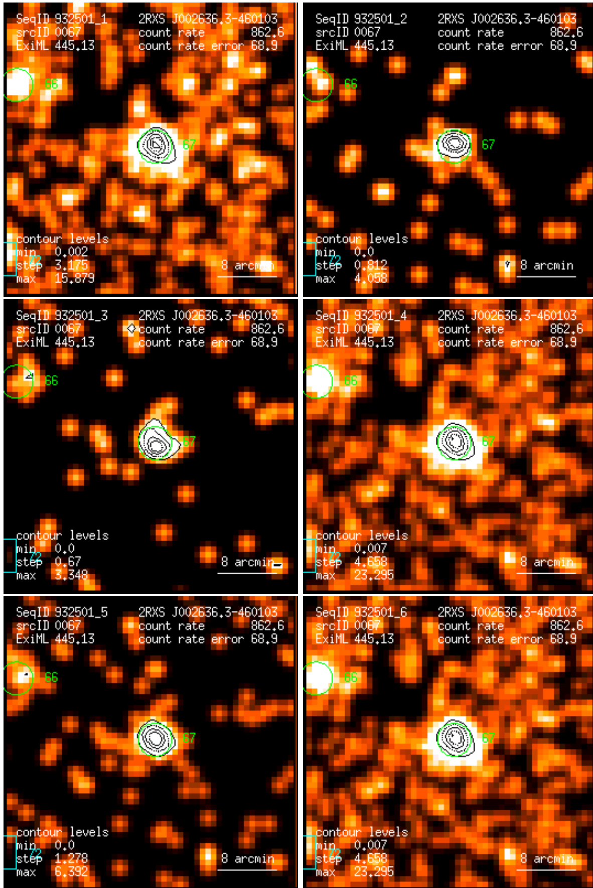
Figure 67: RASS 932501: detection 0067: band rate images, Gaussian filter: (1) PSPC channels 11 – 41, (2) 52 – 90, (3) 91 – 201, (4) 11 – 235, (5) 52 – 201, (6) 11 – 201. Broad band rates in counts/ks. Band rate contour levels in counts/ks/arcmin 2 .
