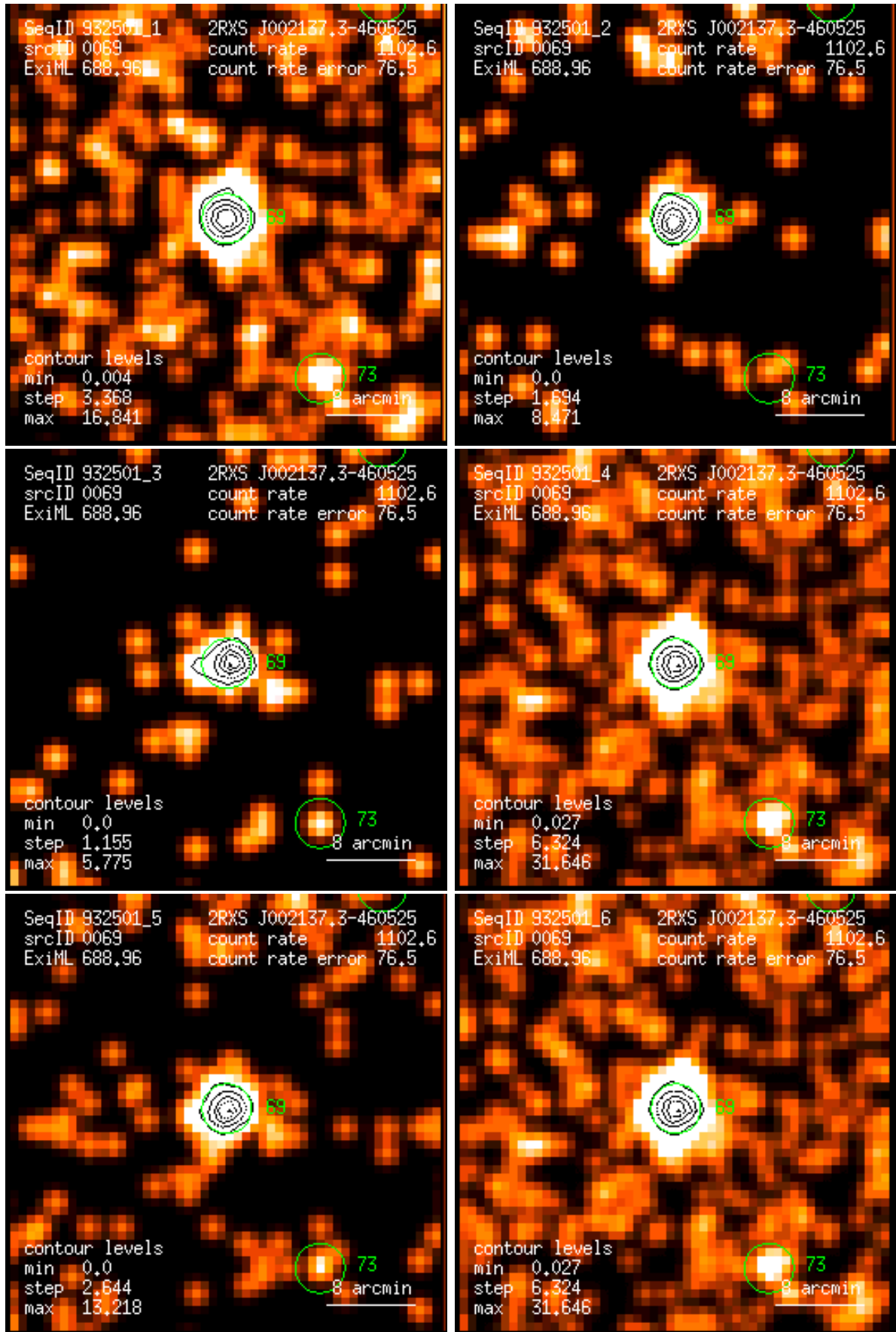
Figure 69: RASS 932501: detection 0069: band rate images, Gaussian filter: (1) PSPC channels 11 – 41, (2) 52 – 90, (3) 91 – 201, (4) 11 – 235, (5) 52 – 201, (6) 11 – 201. Broad band rates in counts/ks. Band rate contour levels in counts/ks/arcmin 2 .
