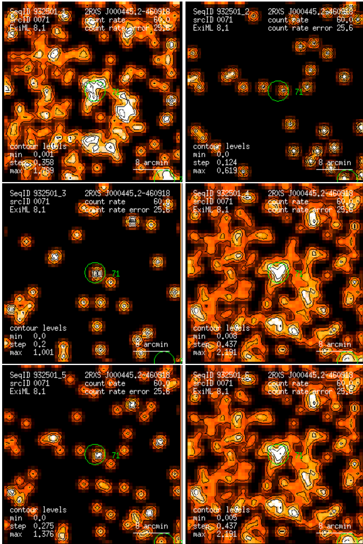
Figure 71: RASS 932501: detection 0071: band rate images, Gaussian filter: (1) PSPC channels 11 – 41, (2) 52 – 90, (3) 91 – 201, (4) 11 – 235, (5) 52 – 201, (6) 11 – 201. Broad band rates in counts/ks. Band rate contour levels in counts/ks/arcmin 2 .
