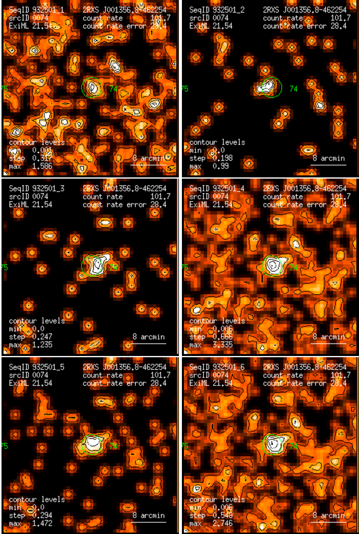
Figure 74: RASS 932501: detection 0074: band rate images, Gaussian filter: (1) PSPC channels 11 – 41, (2) 52 – 90, (3) 91 – 201, (4) 11 – 235, (5) 52 – 201, (6) 11 – 201. Broad band rates in counts/ks. Band rate contour levels in counts/ks/arcmin 2 .
