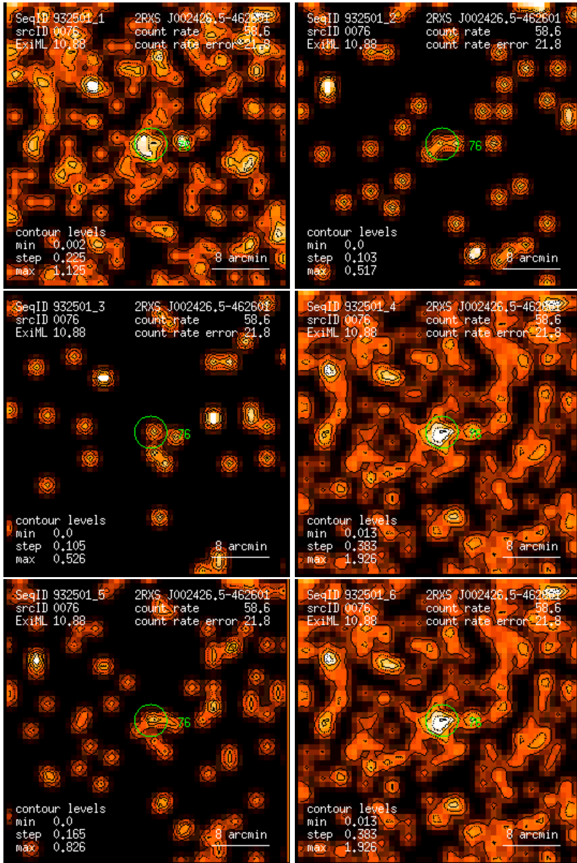
Figure 76: RASS 932501: detection 0076: band rate images, Gaussian filter: (1) PSPC channels 11 – 41, (2) 52 – 90, (3) 91 – 201, (4) 11 – 235, (5) 52 – 201, (6) 11 – 201. Broad band rates in counts/ks. Band rate contour levels in counts/ks/arcmin 2 .
