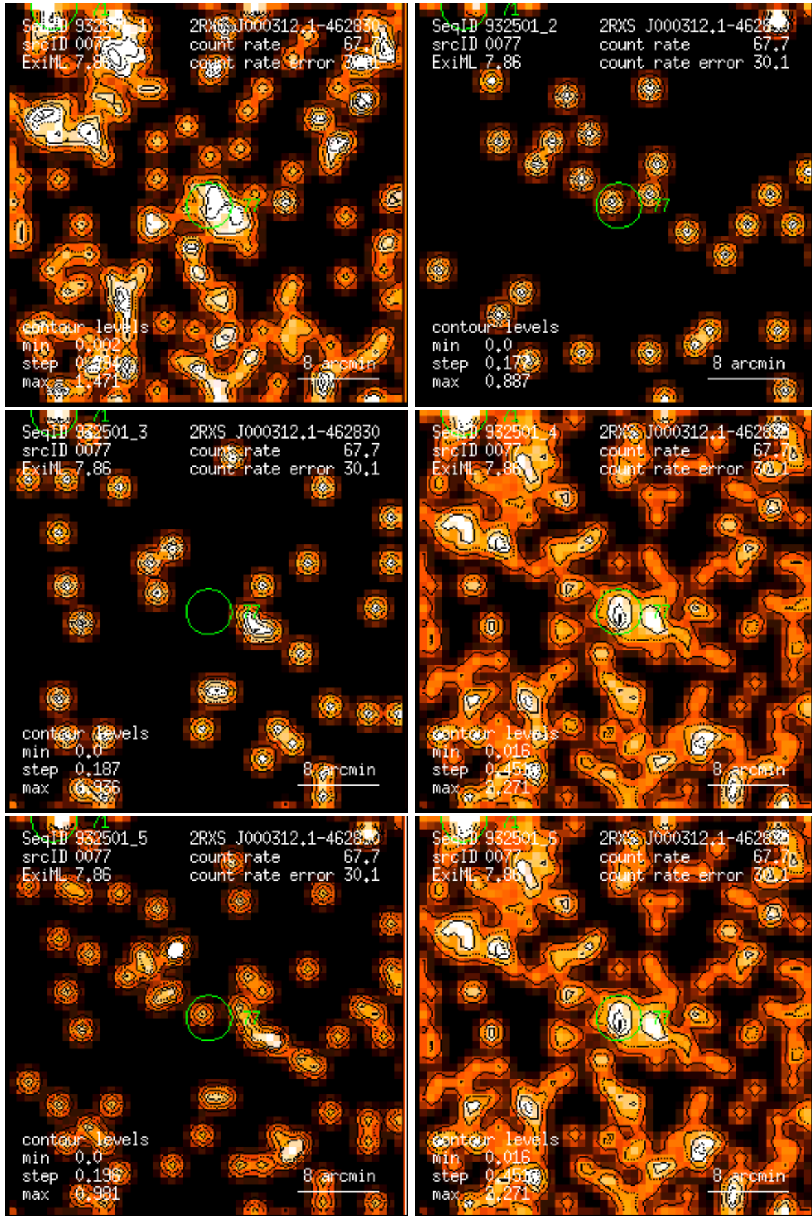
Figure 77: RASS 932501: detection 0077: band rate images, Gaussian filter: (1) PSPC channels 11 – 41, (2) 52 – 90, (3) 91 – 201, (4) 11 – 235, (5) 52 – 201, (6) 11 – 201. Broad band rates in counts/ks. Band rate contour levels in counts/ks/arcmin 2 .
