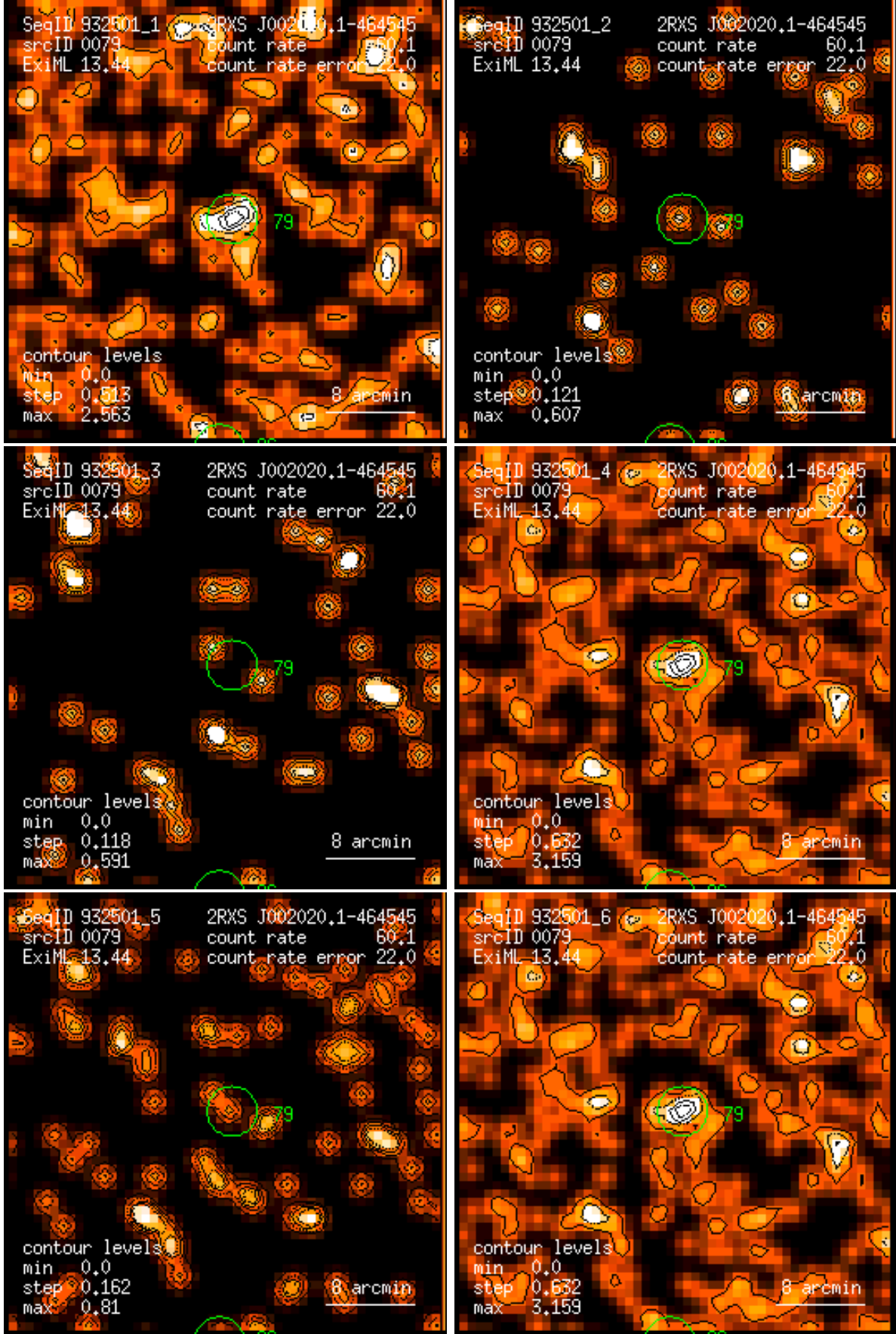
Figure 79: RASS 932501: detection 0079: band rate images, Gaussian filter: (1) PSPC channels 11 – 41, (2) 52 – 90, (3) 91 – 201, (4) 11 – 235, (5) 52 – 201, (6) 11 – 201. Broad band rates in counts/ks. Band rate contour levels in counts/ks/arcmin 2 .
