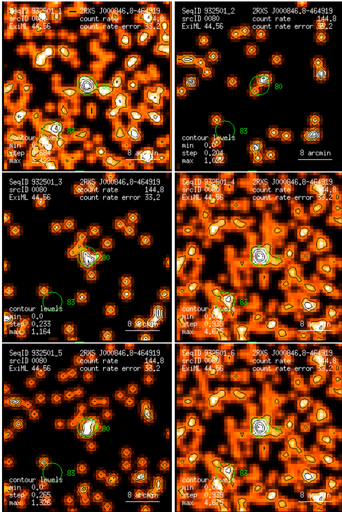
Figure 80: RASS 932501: detection 0080: band rate images, Gaussian filter: (1) PSPC channels 11 – 41, (2) 52 – 90, (3) 91 – 201, (4) 11 – 235, (5) 52 – 201, (6) 11 – 201. Broad band rates in counts/ks. Band rate contour levels in counts/ks/arcmin 2 .
