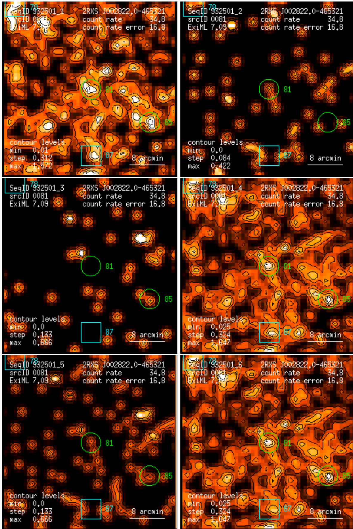
Figure 81: RASS 932501: detection 0081: band rate images, Gaussian filter: (1) PSPC channels 11 – 41, (2) 52 – 90, (3) 91 – 201, (4) 11 – 235, (5) 52 – 201, (6) 11 – 201. Broad band rates in counts/ks. Band rate contour levels in counts/ks/arcmin 2 .
