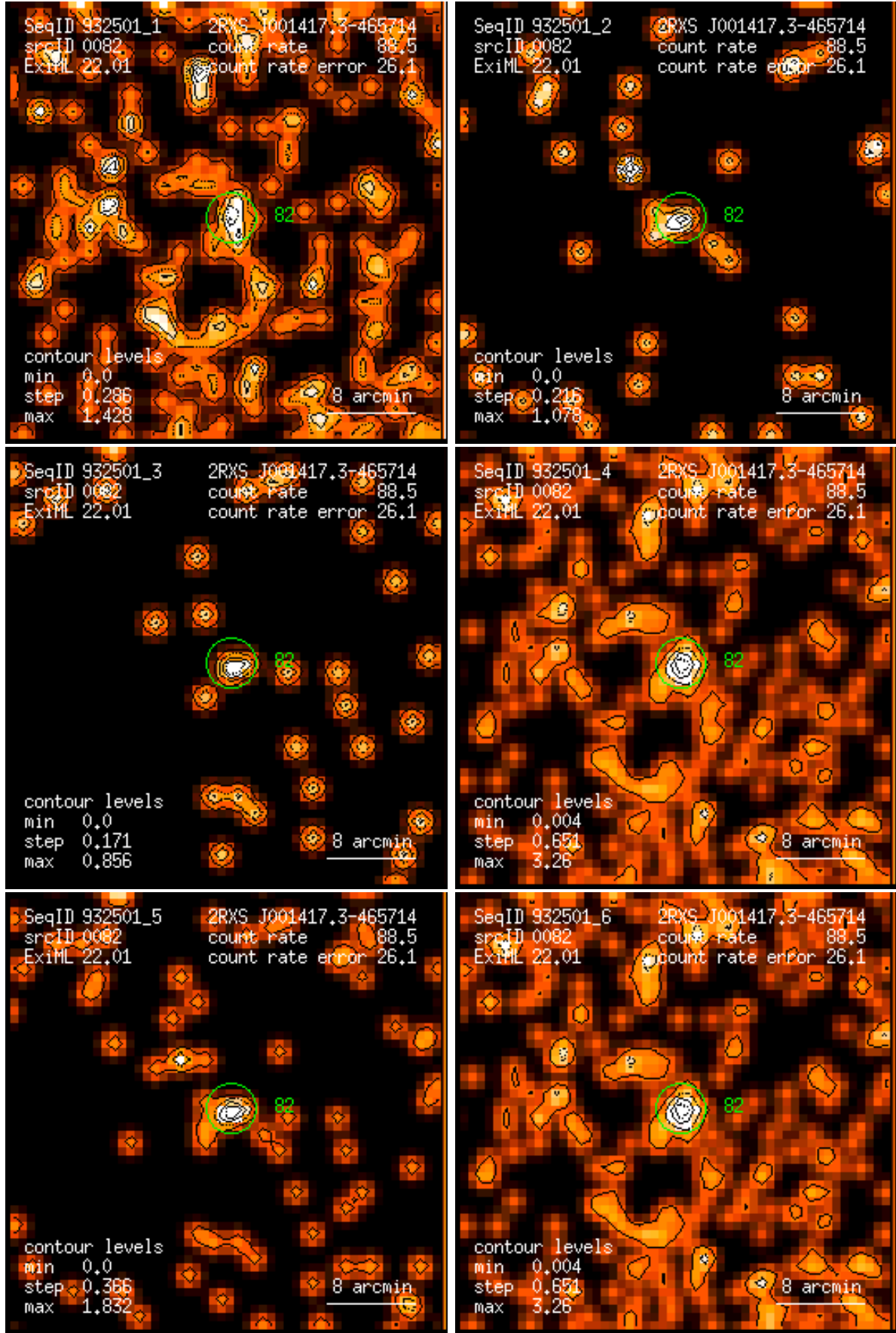
Figure 82: RASS 932501: detection 0082: band rate images, Gaussian filter: (1) PSPC channels 11 – 41, (2) 52 – 90, (3) 91 – 201, (4) 11 – 235, (5) 52 – 201, (6) 11 – 201. Broad band rates in counts/ks. Band rate contour levels in counts/ks/arcmin 2 .
