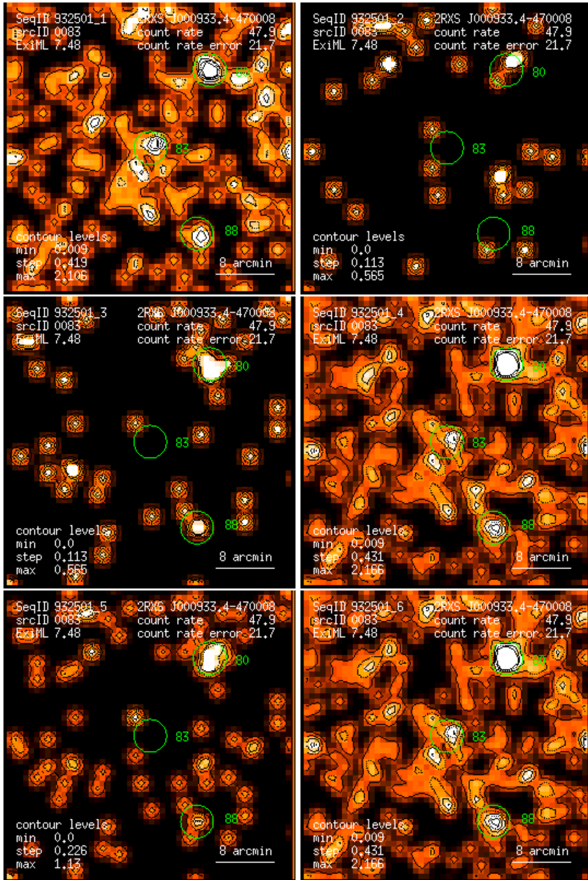
Figure 83: RASS 932501: detection 0083: band rate images, Gaussian filter: (1) PSPC channels 11 – 41, (2) 52 – 90, (3) 91 – 201, (4) 11 – 235, (5) 52 – 201, (6) 11 – 201. Broad band rates in counts/ks. Band rate contour levels in counts/ks/arcmin 2 .
