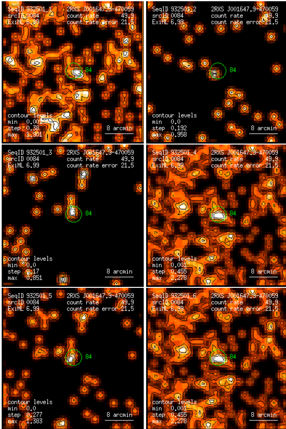
Figure 84: RASS 932501: detection 0084: band rate images, Gaussian filter: (1) PSPC channels 11 – 41, (2) 52 – 90, (3) 91 – 201, (4) 11 – 235, (5) 52 – 201, (6) 11 – 201. Broad band rates in counts/ks. Band rate contour levels in counts/ks/arcmin 2 .
