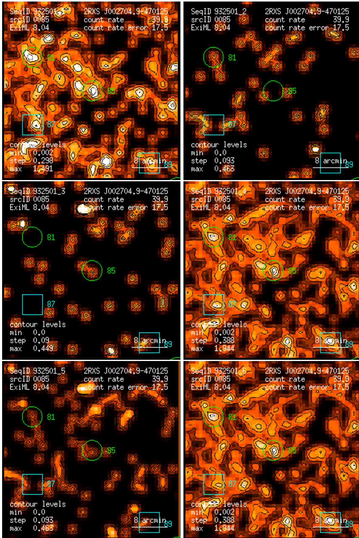
Figure 85: RASS 932501: detection 0085: band rate images, Gaussian filter: (1) PSPC channels 11 – 41, (2) 52 – 90, (3) 91 – 201, (4) 11 – 235, (5) 52 – 201, (6) 11 – 201. Broad band rates in counts/ks. Band rate contour levels in counts/ks/arcmin 2 .
