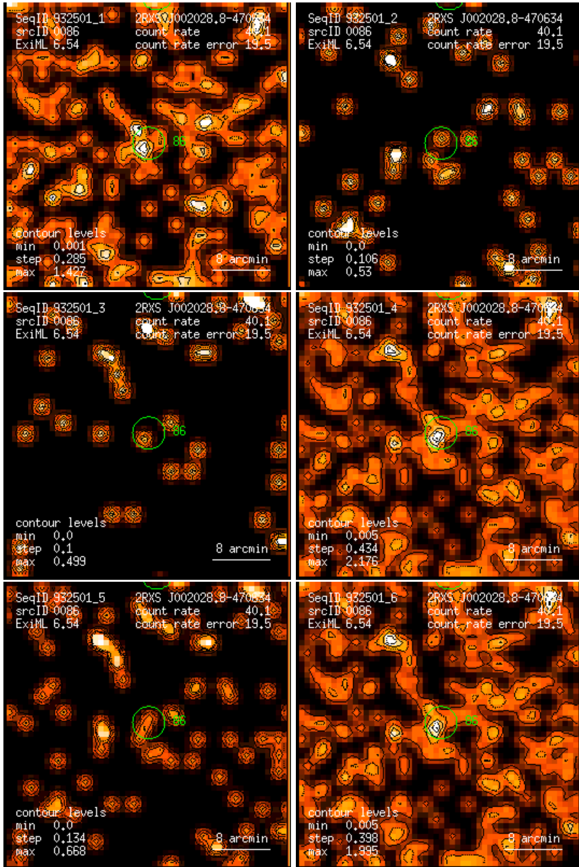
Figure 86: RASS 932501: detection 0086: band rate images, Gaussian filter: (1) PSPC channels 11 – 41, (2) 52 – 90, (3) 91 – 201, (4) 11 – 235, (5) 52 – 201, (6) 11 – 201. Broad band rates in counts/ks. Band rate contour levels in counts/ks/arcmin 2 .
