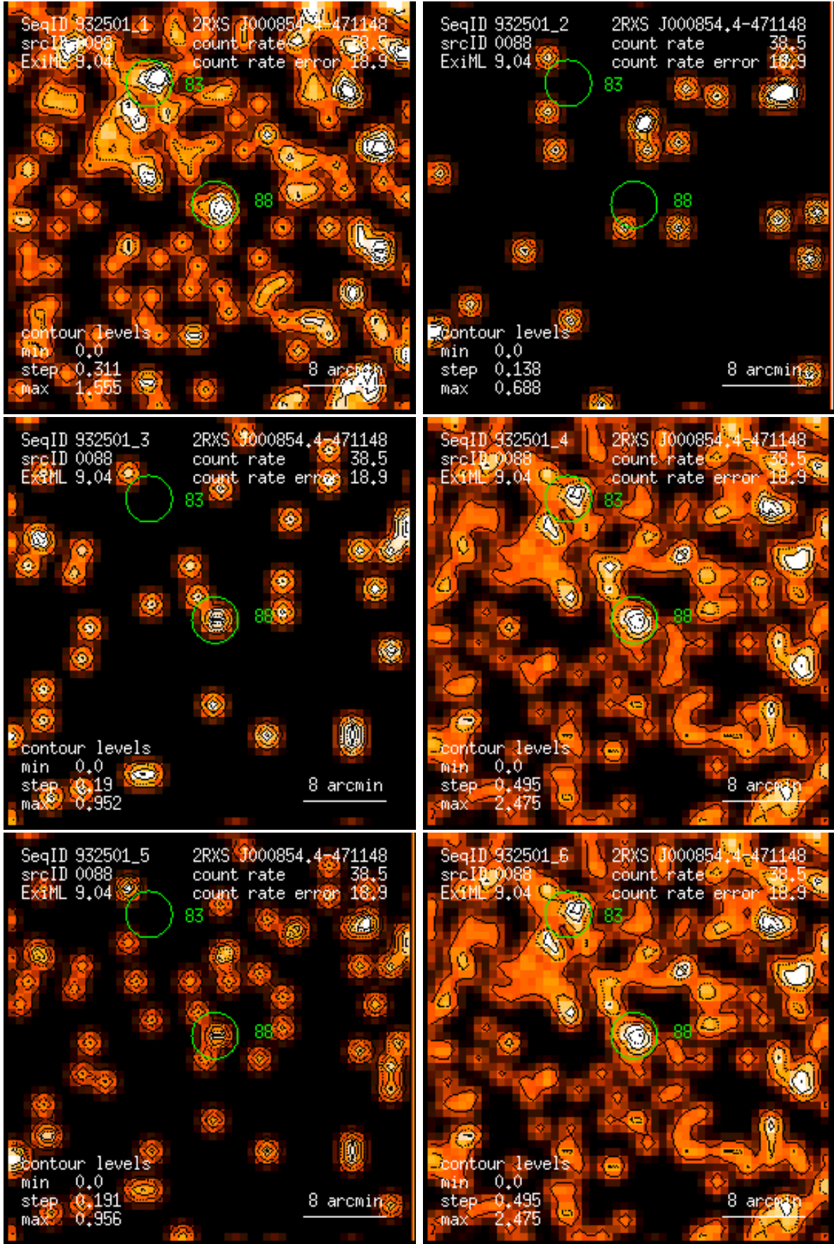
Figure 88: RASS 932501: detection 0088: band rate images, Gaussian filter: (1) PSPC channels 11 – 41, (2) 52 – 90, (3) 91 – 201, (4) 11 – 235, (5) 52 – 201, (6) 11 – 201. Broad band rates in counts/ks. Band rate contour levels in counts/ks/arcmin 2 .
