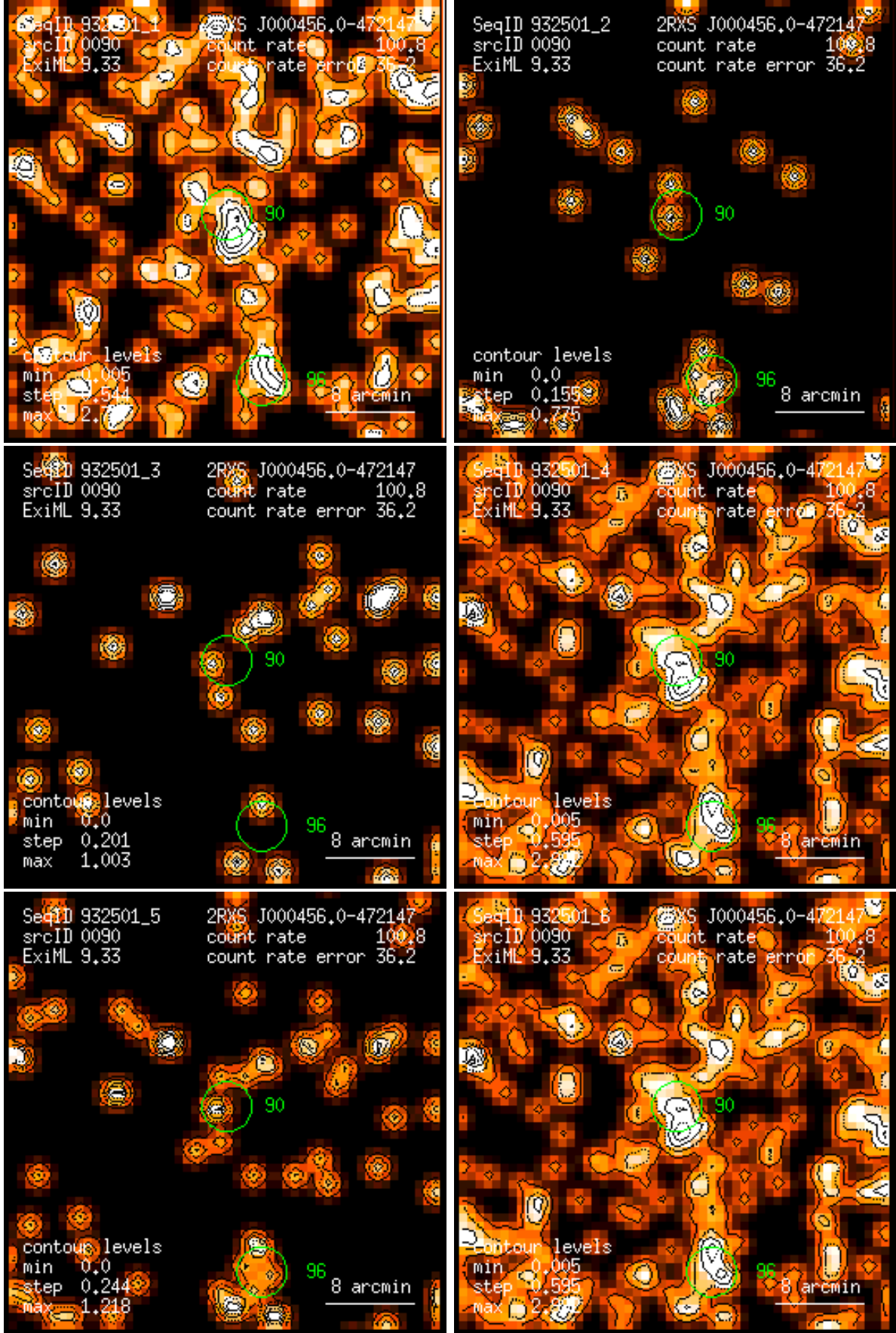
Figure 90: RASS 932501: detection 0090: band rate images, Gaussian filter: (1) PSPC channels 11 – 41, (2) 52 – 90, (3) 91 – 201, (4) 11 – 235, (5) 52 – 201, (6) 11 – 201. Broad band rates in counts/ks. Band rate contour levels in counts/ks/arcmin 2 .
