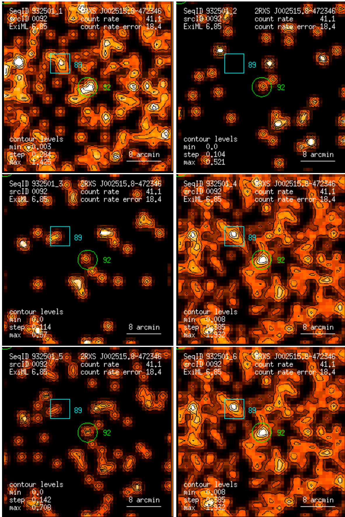
Figure 92: RASS 932501: detection 0092: band rate images, Gaussian filter: (1) PSPC channels 11 – 41, (2) 52 – 90, (3) 91 – 201, (4) 11 – 235, (5) 52 – 201, (6) 11 – 201. Broad band rates in counts/ks. Band rate contour levels in counts/ks/arcmin 2 .
