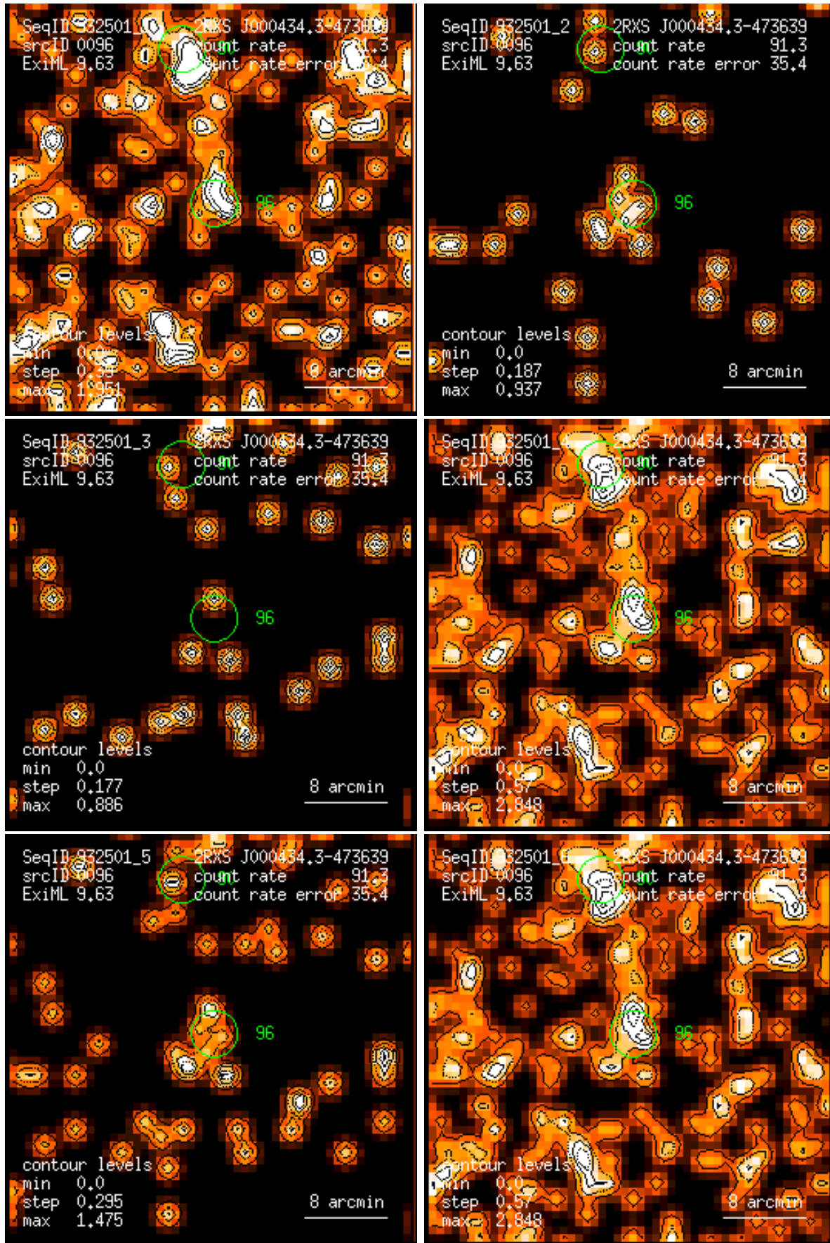
Figure 96: RASS 932501: detection 0096: band rate images, Gaussian filter: (1) PSPC channels 11 – 41, (2) 52 – 90, (3) 91 – 201, (4) 11 – 235, (5) 52 – 201, (6) 11 – 201. Broad band rates in counts/ks. Band rate contour levels in counts/ks/arcmin 2 .
