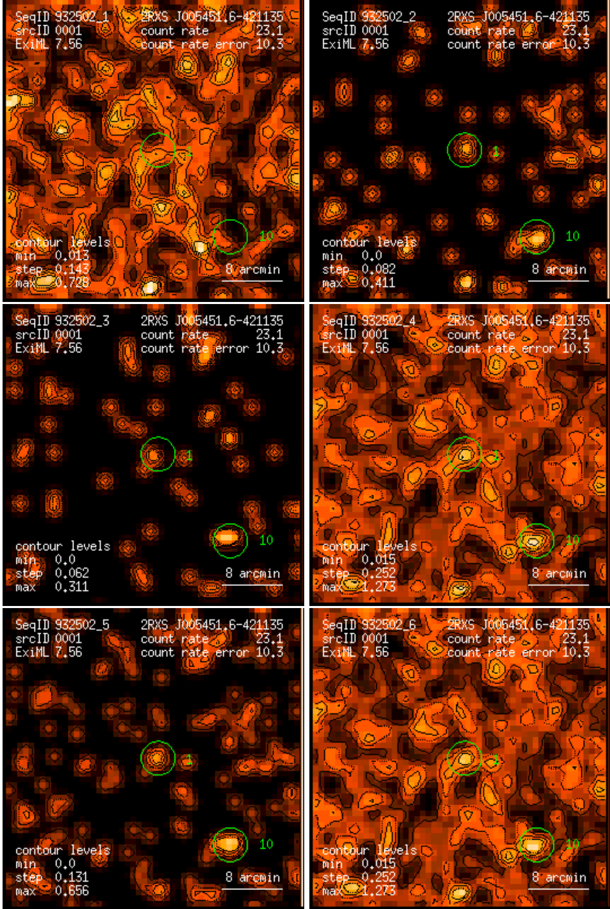
Figure 1: RASS 932502: detection 0001: band rate images, Gaussian filter: (1) PSPC channels 11 – 41, (2) 52 – 90, (3) 91 – 201, (4) 11 – 235, (5) 52 – 201, (6) 11 – 201. Broad band rates in counts/ks. Band rate contour levels in counts/ks/arcmin 2 .
