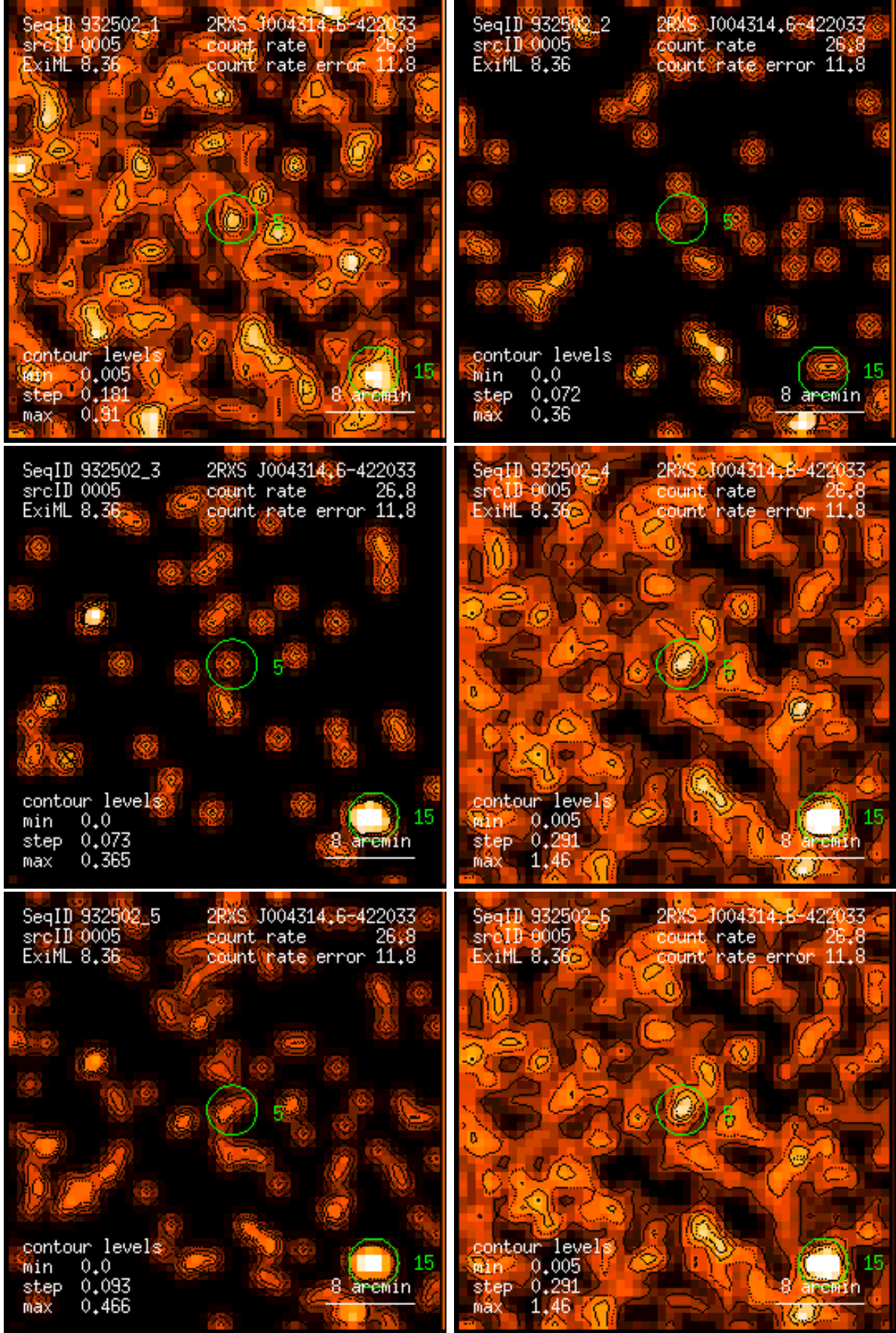
Figure 5: RASS 932502: detection 0005: band rate images, Gaussian filter: (1) PSPC channels 11 – 41, (2) 52 – 90, (3) 91 – 201, (4) 11 – 235, (5) 52 – 201, (6) 11 – 201. Broad band rates in counts/ks. Band rate contour levels in counts/ks/arcmin 2 .
