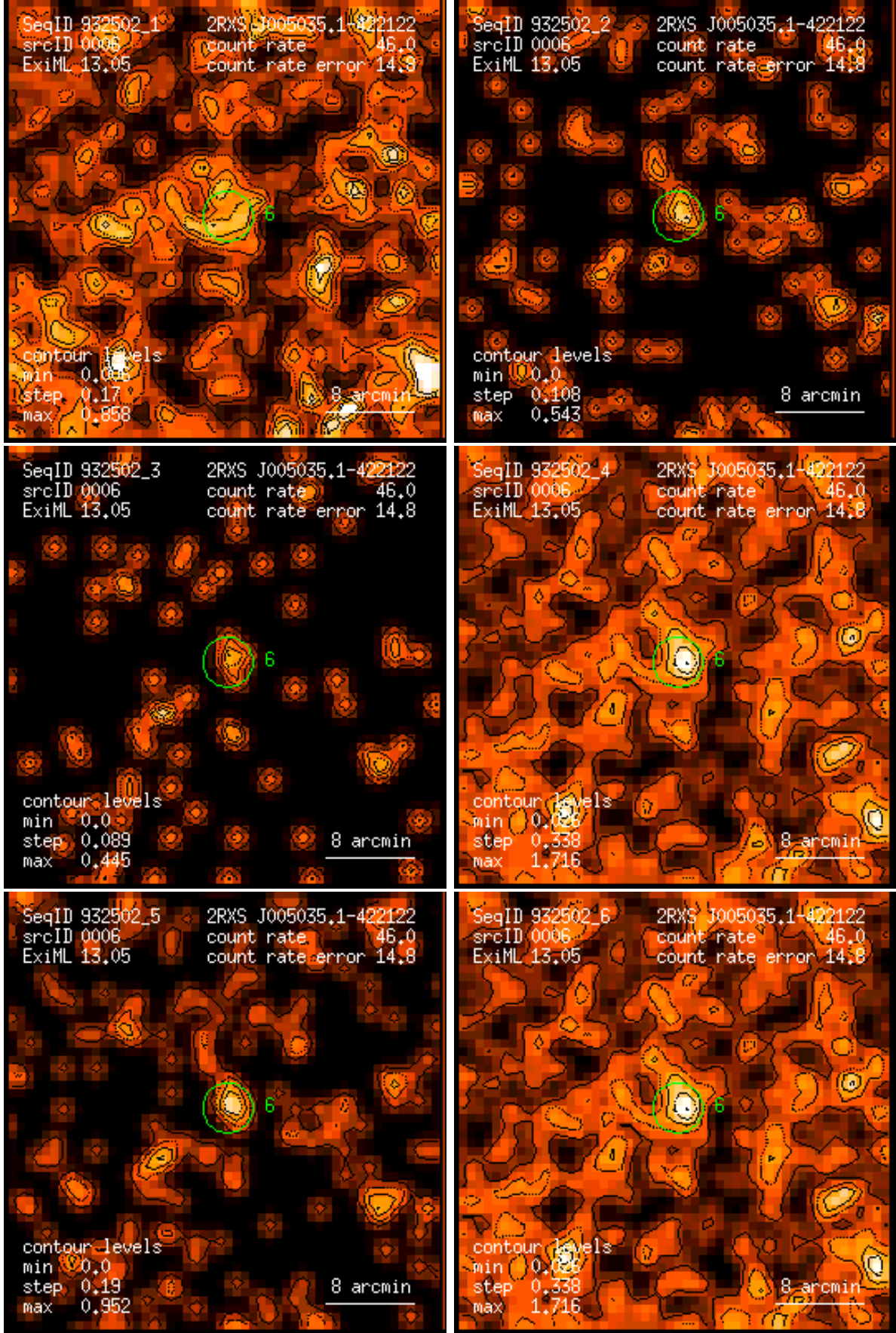
Figure 6: RASS 932502: detection 0006: band rate images, Gaussian filter: (1) PSPC channels 11 – 41, (2) 52 – 90, (3) 91 – 201, (4) 11 – 235, (5) 52 – 201, (6) 11 – 201. Broad band rates in counts/ks. Band rate contour levels in counts/ks/arcmin 2 .
