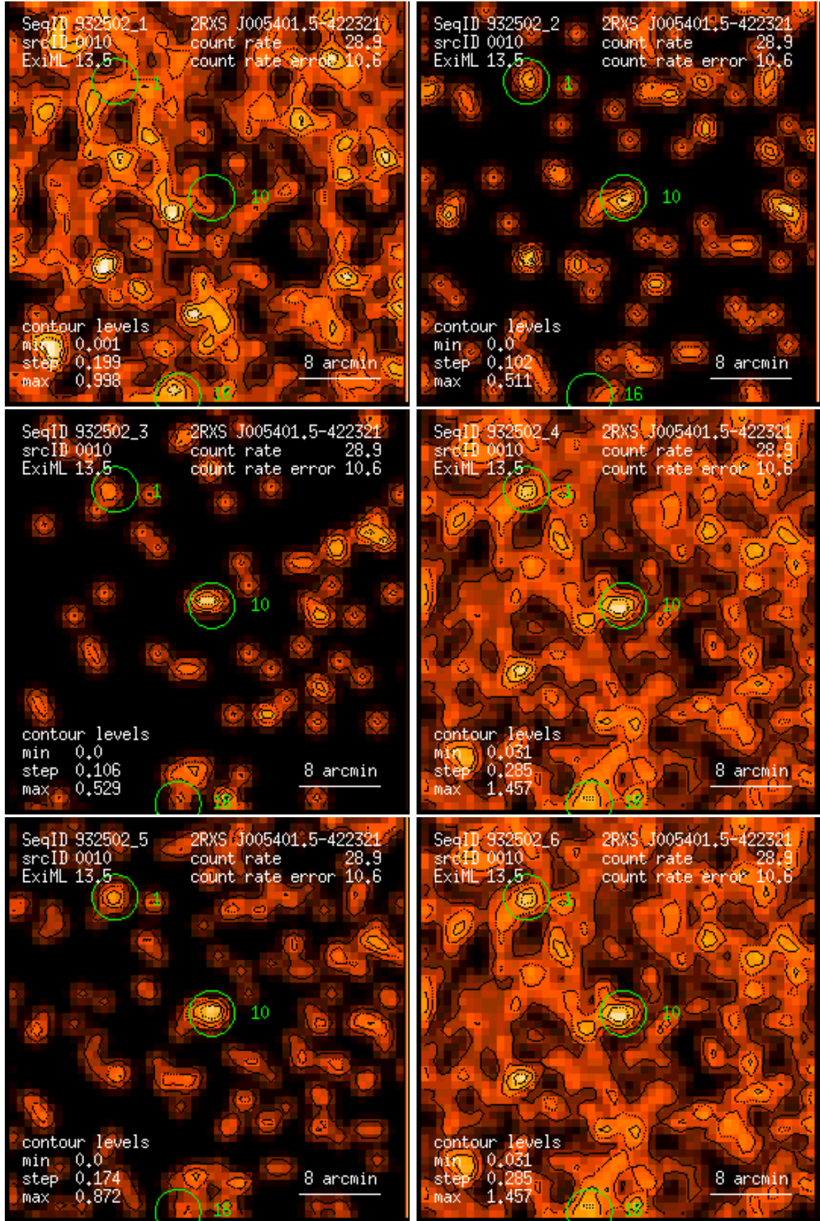
Figure 10: RASS 932502: detection 0010: band rate images, Gaussian filter: (1) PSPC channels 11 – 41, (2) 52 – 90, (3) 91 – 201, (4) 11 – 235, (5) 52 – 201, (6) 11 – 201. Broad band rates in counts/ks. Band rate contour levels in counts/ks/arcmin 2 .
