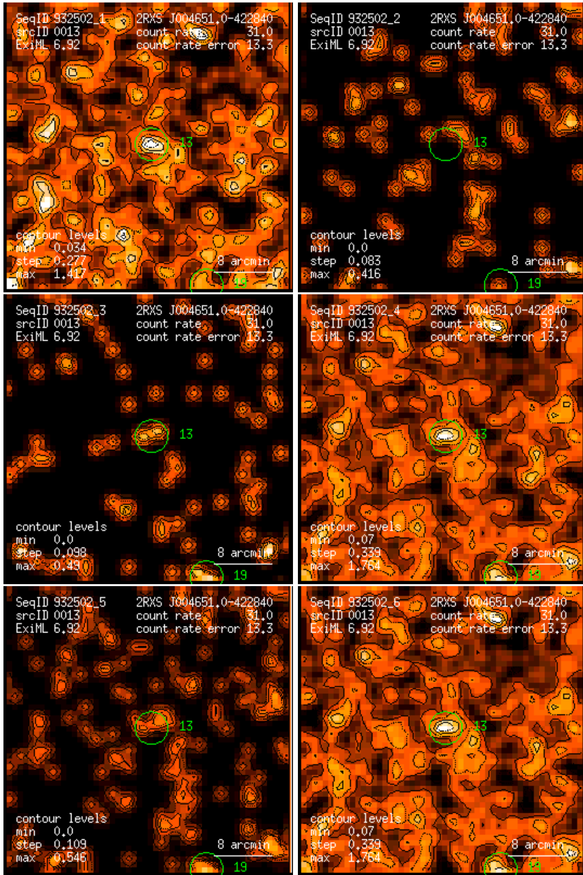
Figure 13: RASS 932502: detection 0013: band rate images, Gaussian filter: (1) PSPC channels 11 – 41, (2) 52 – 90, (3) 91 – 201, (4) 11 – 235, (5) 52 – 201, (6) 11 – 201. Broad band rates in counts/ks. Band rate contour levels in counts/ks/arcmin 2 .
